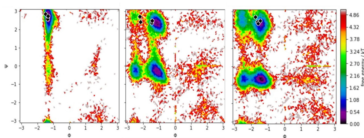
Figure 4 : Ramachandran Plot and free energy plot generated for Proline, Serine and Aspartate residues from the MD simulations and coordinates of the bound peptide from complexes are superimposed as black (+) signs
