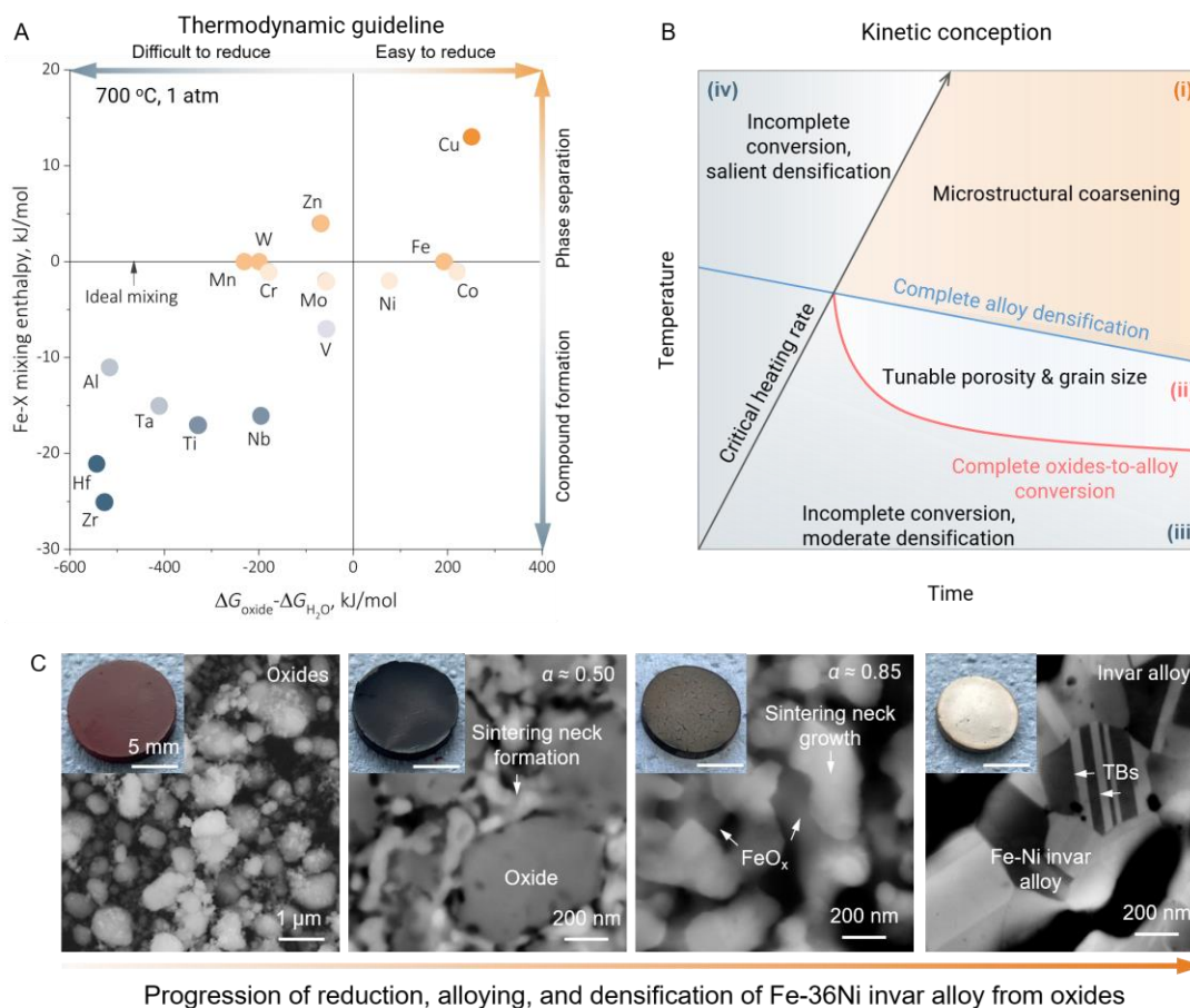
Figure 5 | The concept of one-step synthesis of bulk HEM from oxides. A. Thermodynamic design guidelines considering the bulk reducibility and substitutional alloying capability. B. Kinetic conception sketching the possible microstructure states while considering the temperature, time, and conversion rate. C. Microstructure evolution during the synthesis of bulk Fe-36Ni invar alloys from Fe 2 O 3 and NiO using H 2 . Figure reproduced with permission from Ref. (102).
