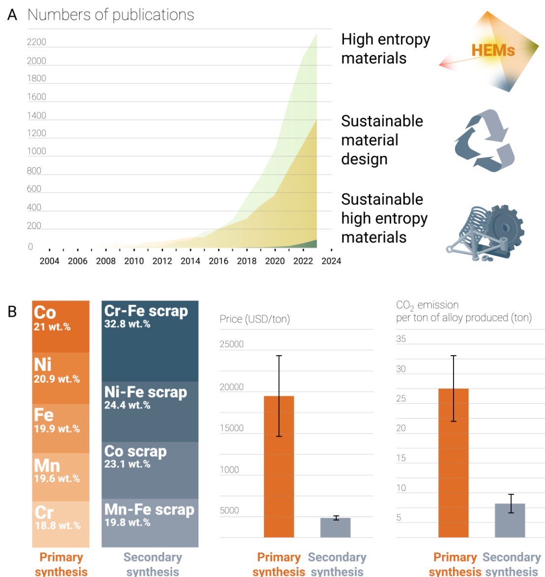
Figure 2. Increasing interest in sustainable high entropy materials design. A Increase in scientific literature output on “high entropy materials,” “sustainable material design,” and “sustainable high entropy materials.” B Comparison of some real-world key metrics considering the required raw materials for the CoCrFeNiMn (Cantor) alloy when fabricated via primary synthesis (high-purity metallic materials from minerals) and secondary synthesis (from scrap). The analysis shows the average values for the price and CO 2 footprint.
