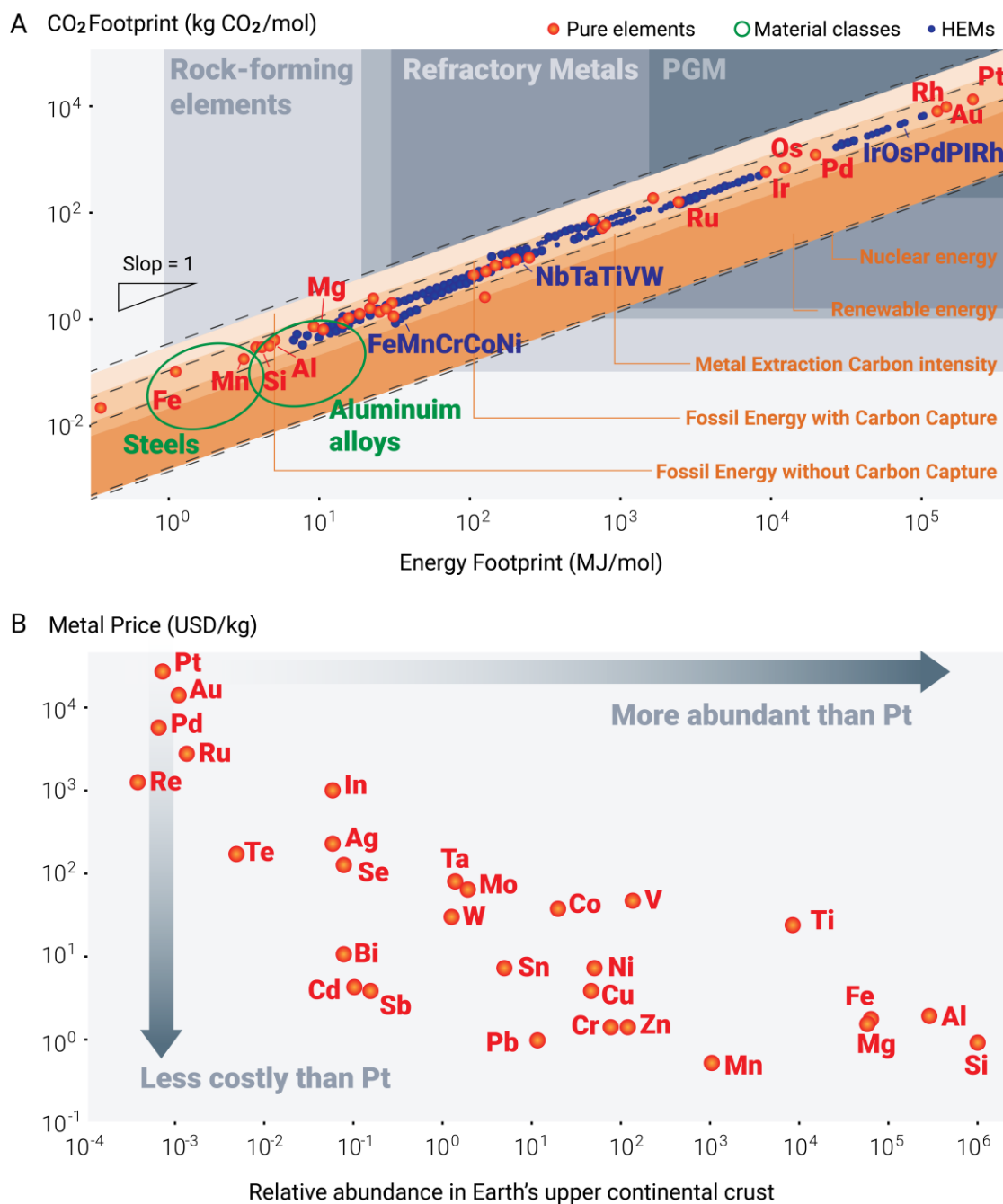
Figure 1. Energy-, carbon-, cost-, abundance considerations of high entropy materials and metals. A CO 2 footprint associated with the energy required for the metal extraction of more than 30,000 different HEMs (blue dots). The values of pure metals (red dots) and larger material classes, such as steels and aluminum alloys (green circles), are also shown as Ref. (61). B Relationship between metal prices and the relative abundance of chemical elements in the Earth's upper continental crust on the basis of the abundance of silicon with 10 6 atoms(62). Notably, not only the abundance but also the dispersion (richness) across a larger scale and within the ore minerals determines the CO 2 and energy footprints of metal extraction. PGM: Platinum Group Metal.
