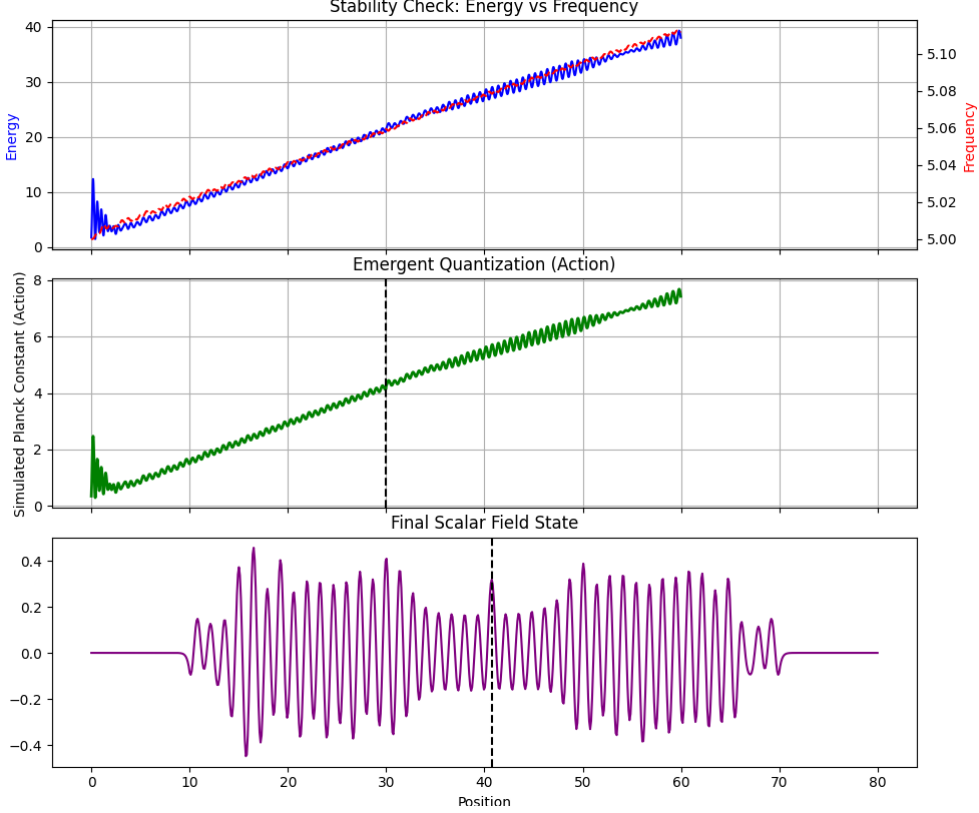
Figure 2: Dynamics of Action and Vacuum State. Top: Under acceleration, the particle interacts with varying vacuum potential, causing the internal frequency to adjust. Middle: The simulated action ( \hbar_{eff} = E/\Omega ) is observed to evolve. This is consistent with the model's core premise: while the geometric scaling law (governed by e ) is fundamental and invariant, the effective Planck constant is a dynamic variable determined by the local vacuum density D . Bottom: Snapshot of the scalar field packet.
