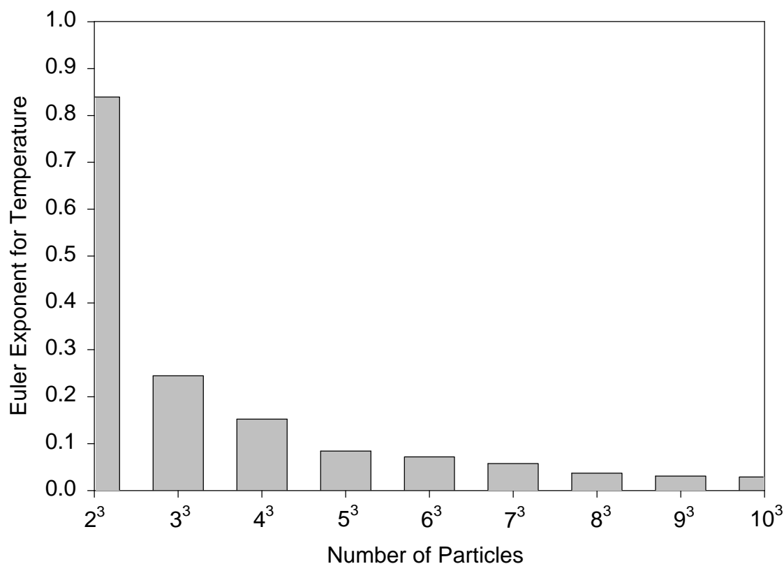
Figure 3 - Euler exponent for temperature as a function of system size.
