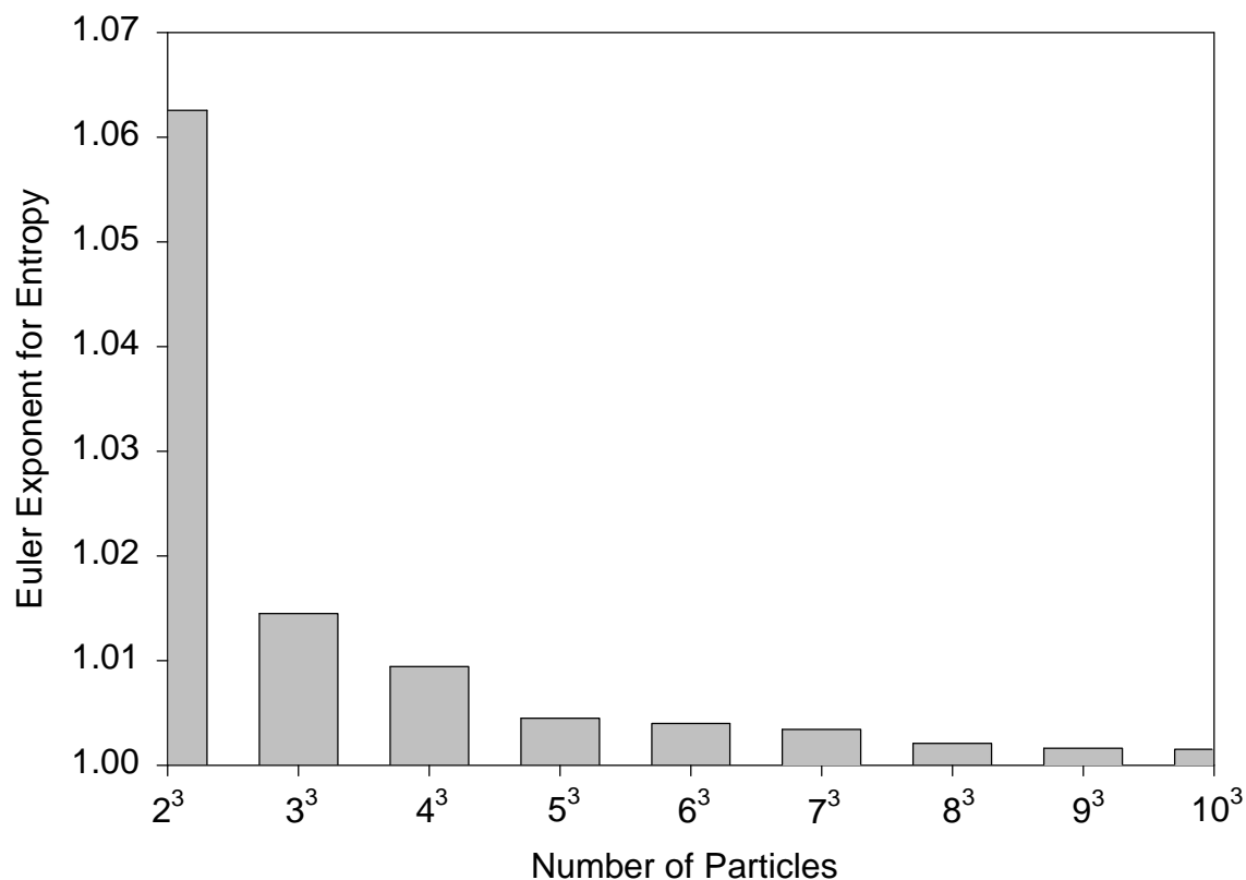
Figure 2 - Euler exponent for entropy as a function of system size.
