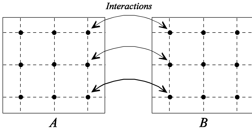
Figure 5 - When two systems combine, cross interactions of the particles, especially those near the joining region, reduce the internal potential energy of the combined system.
