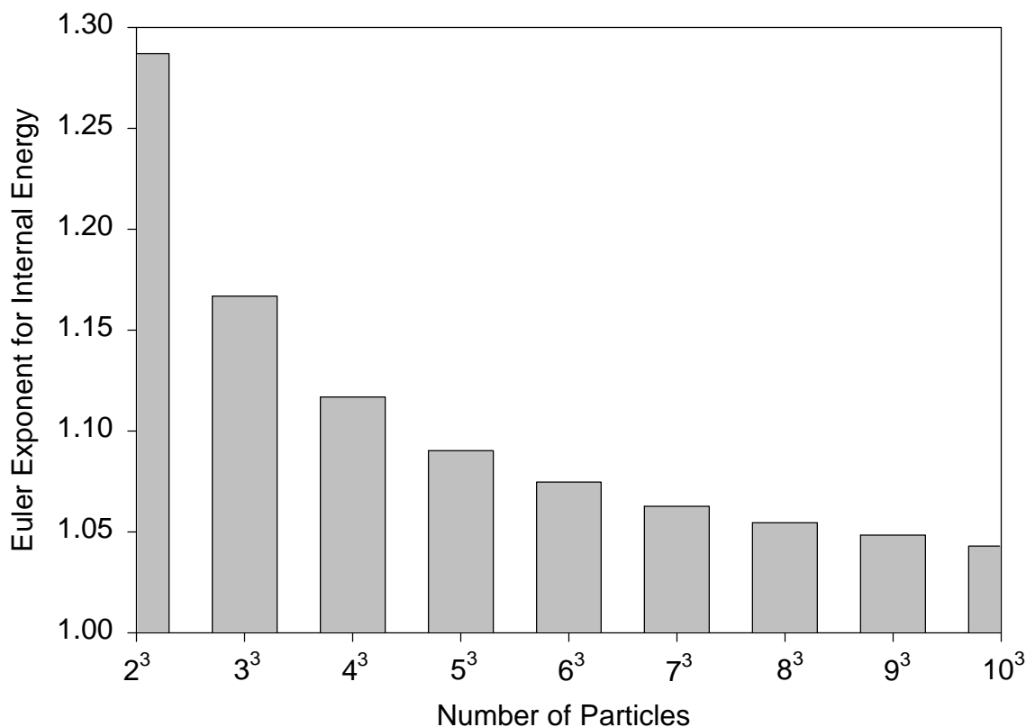
Figure 1 - Euler exponent for internal energy as a function of system size.
