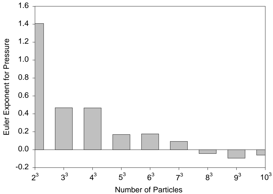
Figure 4 - Euler exponent for pressure as a function of system size.
