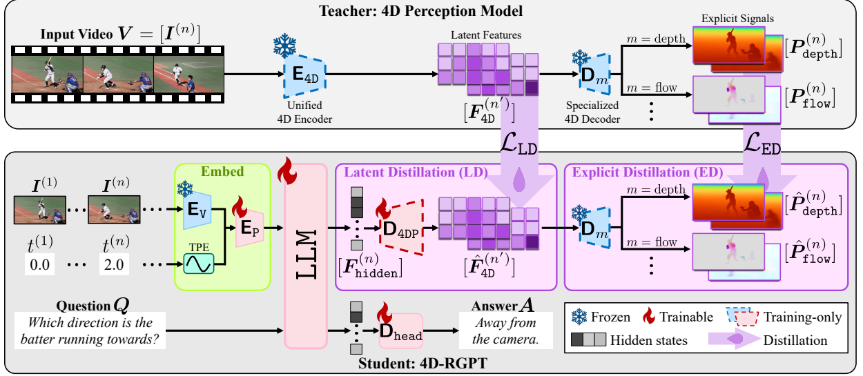
Figure 2 | Perceptual 4D Distillation (P4D) framework for 4D-RGPT. For each frame I^{(i)} in V , 4D-RGPT extracts 4D representations through training-only modules, i.e. , D_{4DP} and D_m for m \in \mathcal{M} . This includes both latent features, i.e. , \hat{F}_{4D} , and explicit signals, e.g. , depth \hat{P}_{\text{depth}} or optical flow maps \hat{P}_{\text{flow}} . We also incorporate timestamp positional encodings (TPE) to provide temporal cues for 4D-RGPT to be temporally aware. In the P4D framework, the frozen teacher, i.e. , 4D perception model, captures 4D expert knowledge from V . It is then distilled to the student 4D-RGPT via two strategies. (a) Latent Distillation (LD) : We align the latent \hat{F}_{4D} with the teacher’s intermediate 4D embeddings F_{4D} . (b) Explicit Distillation (ED) : We align the explicit \hat{P}_m with the teacher’s final 4D signals P_m . 4D-RGPT is optimized end-to-end using both SFT loss and the distillation losses, i.e. , \mathcal{L}_{LD} and \mathcal{L}_{ED} .
