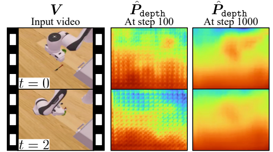
Figure 5 | Predicted depth maps at different training steps. We visualize the progress of \hat{P}_{\text{depth}} throughout training.
