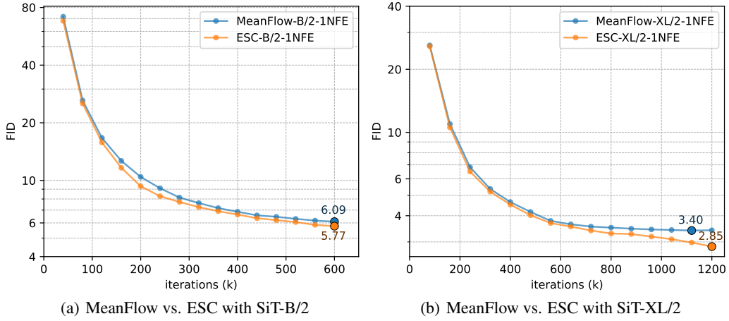
Figure 9: Convergence of FID with different model architectures.
