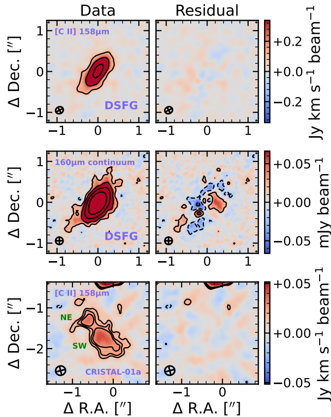
Fig. 2. Results from parametric 2D modeling with PyAutoGALAXY. Each row shows a different source and/or image. Left column displays the observed emission, while the right column shows the residuals after subtracting the maximum likelihood model. The first and second rows show the modeling of the DSFG’s [C II] emission and 160 \mu m dust continuum, respectively. Black contours represent the \pm 3, 9, 27 and 81\sigma levels. Results for the [C II] emission of CRISTAL-01a (CRISTAL-1) are shown in the third row. Here, the contours only trace \pm 3, 4 and 5\sigma levels.
