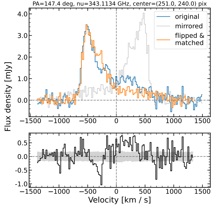
Fig. A.1. Symmetric difference analysis for aperture #1. Upper panel: [C II] spectra of the cropped aperture #1 (blue), its mirrored version (gray), and the mirrored version but velocity-inverted (flipped), shifted and matched to the original peak (orange). Lower panel: Residuals from the difference between the original and the flipped-and-matched spectra.
