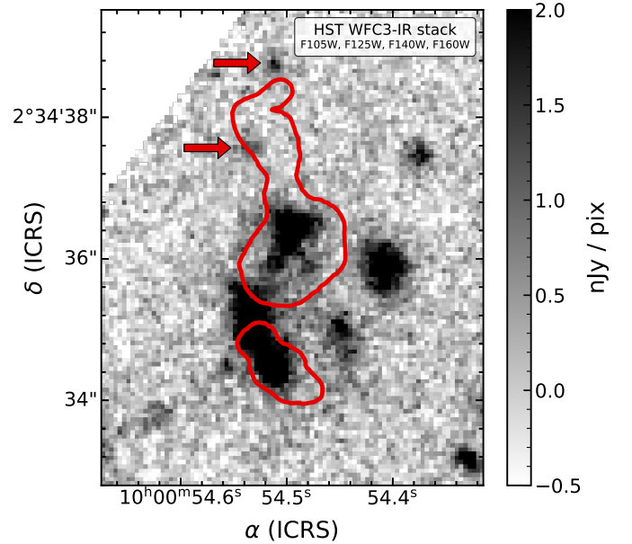
Fig. B.1. Stack of HST/WFC3-IR imaging of J1000+0234 with the outline of the [C II] emission in red. Arrows indicate the positions of the two sources potentially associated with the plume.
