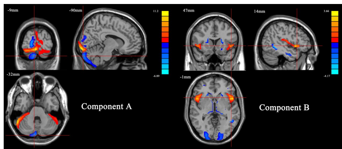
Figure 1. The two components showed significant case/control difference. Component A mainly included bilateral Crus I, left lingual gyrus, left Crus II, and left fusiform (Z score > 2, cluster volume > 1.5 cc 3 ). Component B mainly included bilateral insula, caudate, thalamus and middle occipital gyrus (Z score > 2, cluster volume > 1.5 cc 3 ).
