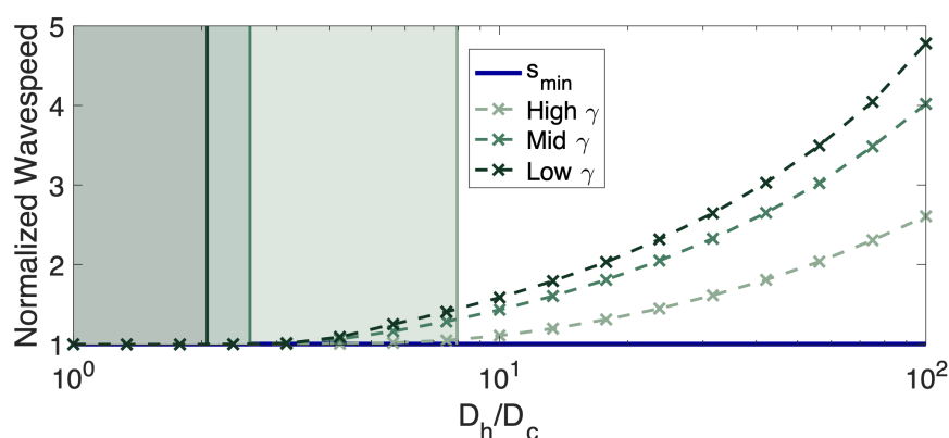
Fig. 4 As D_h/D_c is increased for varying \gamma values, we see an increase in the converged numerical wave-speed that is more pronounced for smaller values of \gamma ; the corresponding thresholds k for wave-speeds faster than s_{min} are indicated. Wave-speeds taken as the average speed between 8 and 8.5cm of growth on simulated T2 MRI (16% total cell density threshold) and presented relative to s_{min} .
