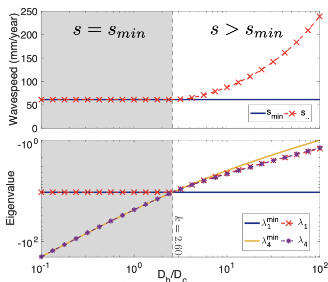
Fig. 2 As D_h/D_c is increased with D_c = 10^{1.5} \text{ mm}^2/\text{year} , \rho = 10^{1.5}/\text{year} and \gamma = 0.05/\text{day} , we see an increase in the converged numerical wave-speed past the threshold on D_h/D_c of k = 2.60 . Wave-speeds taken as the average speed between 8 and 8.5cm of growth on simulated T2 MRI (16% total cell density threshold).
