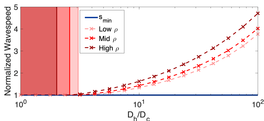
Fig. 5 As D_h/D_c is increased for varying D_c and \rho values, we see an increase in the relative wave-speed s/s_{min} that is more pronounced for larger values of \rho . The observed trend agrees with the expectation given by the corresponding values of k , which are also indicated. Wave-speeds taken as the average speed between 8 and 8.5cm of growth on simulated T2 MRI (16% total cell density threshold) and normalized against s_{min} .
