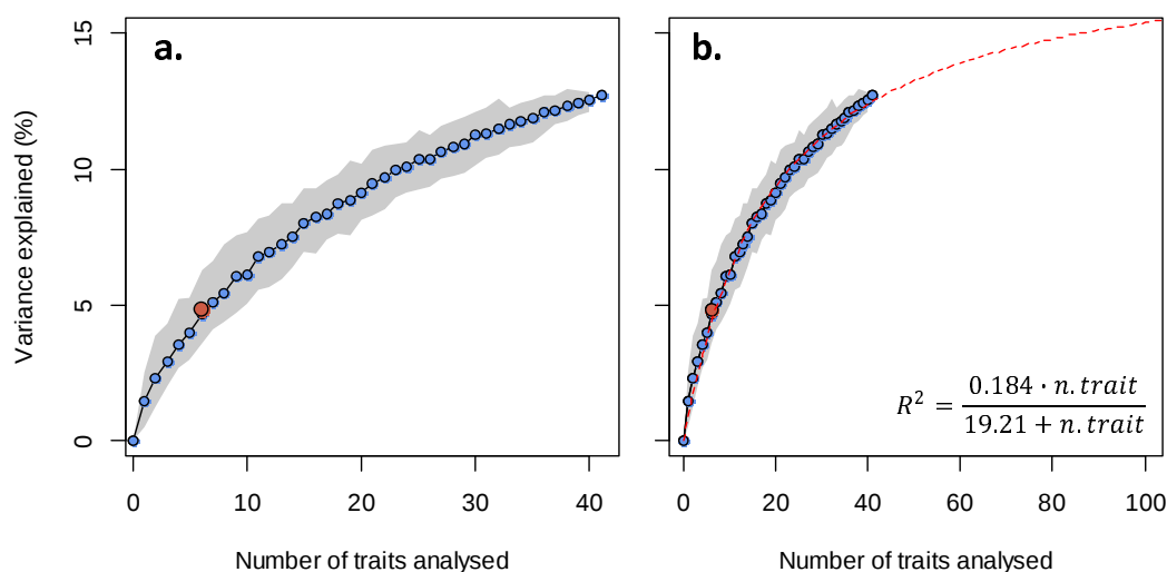
Figure 4. The average proportion of variation in ecosystem functions across years explained by plant traits increases asymptotically with the number of traits included in the analysis. The red dot shows the proportion of explained variation when only the six traits most commonly assessed in other studies are included. A: the marginal R^2 – number of traits relationship based on analysis of actual data. B: an
