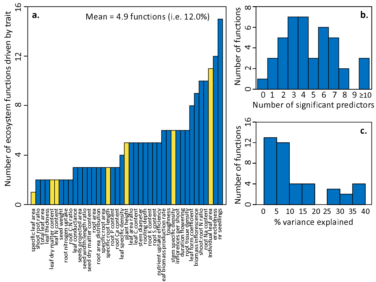
Figure 2. The relative importance of different and multiple traits for ecosystem functioning across years. A: the number of analyzed functions that was significantly driven by each trait, according to final models. The traits analyzed in over 10% of the papers included in the review are shown in yellow. B: Number of significant predictors in final models of each ecosystem function. C: Marginal R^2 values for final models of each ecosystem function.
