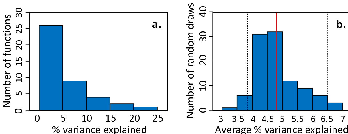
Figure 3. R^2 values of models in which only six traits were analyzed to explain ecosystem functions across years. A: Distribution of marginal R^2 values of final models for each trait, when only the six most frequently investigated traits (see review) were included in the analysis. B: Distribution of mean marginal R^2 values (across final models for each trait), when based on 100 random draws, six randomly selected investigated traits were included in the analysis. The vertical dashed bars show the 95% confidence interval, while the vertical red bar shows the mean marginal R^2 across all functions when only the six most frequently investigated traits were included in the analysis.
