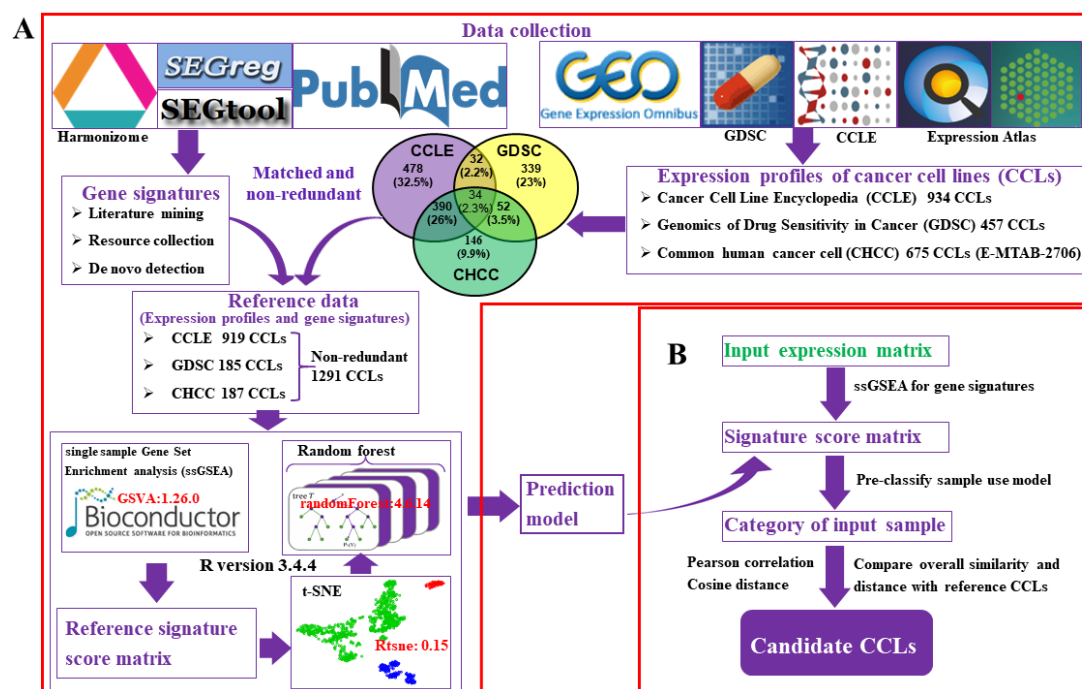
Figure 1 The data resources and algorithm of CCLA. (A) The resource collection and model construction for reference CCLs. The reference data of CCLs in CCLA were from three resources: CCLE, GDSC and CHCC (E-MTAB-2706 dataset in EBI). The gene signatures of CCLs were from three parts: 1) Text mining from publications; 2) SEGs collection from databases; 3) De novo detection by R package SEGtool. (B) The core steps of CCLA algorithm.
