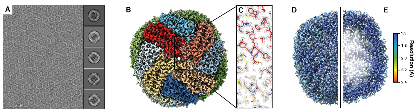
Figure 2. \sim 1.75 Å resolution cryo-EM reconstruction of mouse heavy chain apoferritin. (A). Representative aligned and dose-weighted micrograph (imaged at \sim 1.2 \mu m underfocus) of apoferritin in vitreous ice. Representative reference-free 2D class averages are shown in the right-side inset. (B). Final apoferritin EM density colored by subunit. (C). Zoomed in region of the final apoferritin EM density (gray mesh). Residues are shown in stick representation and colored by subunit according to (B). (D). Final apoferritin EM density colored by local resolution shown in full or (E) sliced in half.
