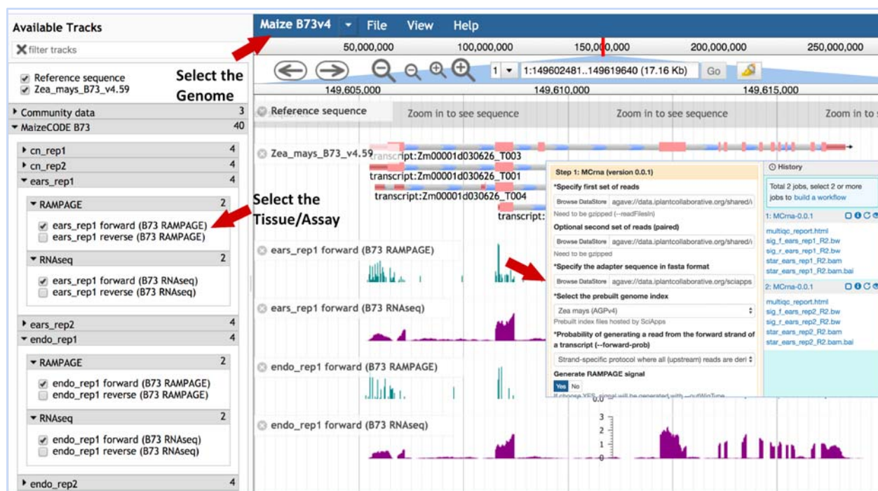
Figure 3. Genome browser tracks for the MaizeCODE data. JBrowse is used to hold the MaizeCODE signal tracks, which are organized in the following order: genome, tissue, replicate, and assay. Clicking on each track brings up the workflow 'Relaunch' interface.
