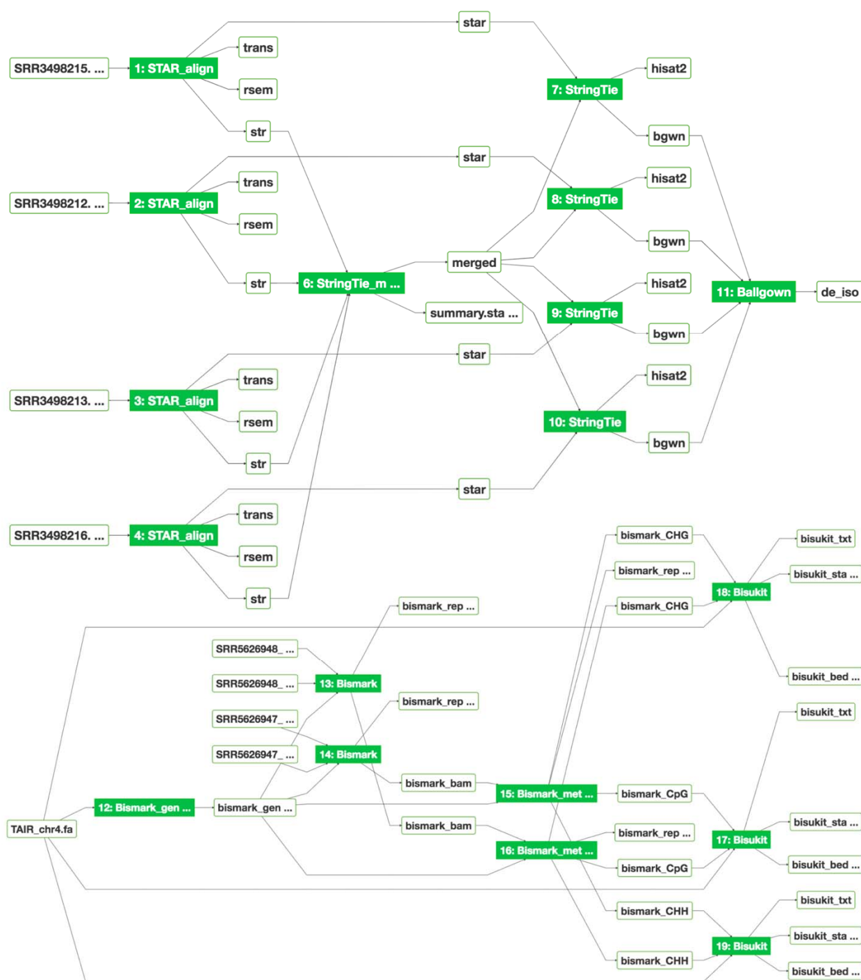
Figure 4. Graphical workflow diagrams for differential expression analysis (top) and MethylationC-seq analysis (bottom). The interactive graph demonstrates the relationships among input–output files, displays provenance of the software tools, and provides real-time job status updates of
