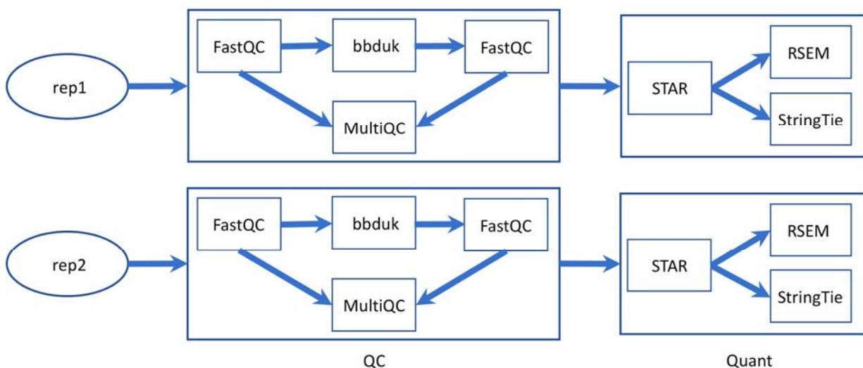
Figure 5. MaizeCODE MCrna app for processing RNA-seq data from two replicates.
