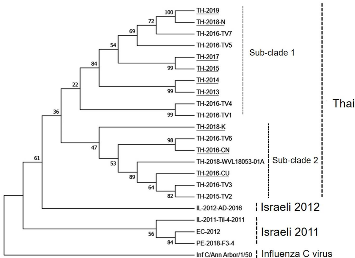
Figure 1 Maximum-likelihood phylogenetic trees based on TiLV genomic segment 1 PB1 nucleotide sequences depicting TiLV being clustered into 3 clades. Isolates with and without underlines represent sequences obtained from this study and those from the GenBank database, respectively. Codes of the viral isolates are listed in Table 1. The influenza C virus sequence was used as outgroup. Percent bootstrap values from 1,000 replications are shown.
