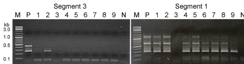
Figure 3 a) Sensitivity tests of two semi-nested RT-PCR protocols (segment 1 and 3) using serial dilutions of RNA from three TiLV-infected fish. A starting 100 ng of RNA from three individual TiLV-infected fish was 10-fold serially diluted and subjected to semi-nested RT-PCR protocols using primers targeting genome segment 3 (Dong et al. 2017b) and segment 1 (this study). M, 2 log DNA marker; N, no template control; #, cross hybridized PCR products. b) Representative comparison tests with 9 archived samples (1-9) obtained from Dong et al. (2020); P, positive control (infected tissue) and N, negative control (no RNA template).
