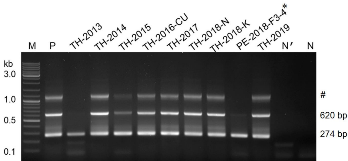
Figure 4 Validation of the newly developed semi-nested RT-PCR assays in detecting TiLV segment 1 from archived samples obtained from years 2013 to 2019. *sample from Peru described in Pulido et al. (2019); M, 2 log DNA marker; P, positive control (infected tissue); TH, samples from Thailand; PE, sample from Peru; N', non-infected fish RNA; N, no template control; #, cross hybridized PCR products.
