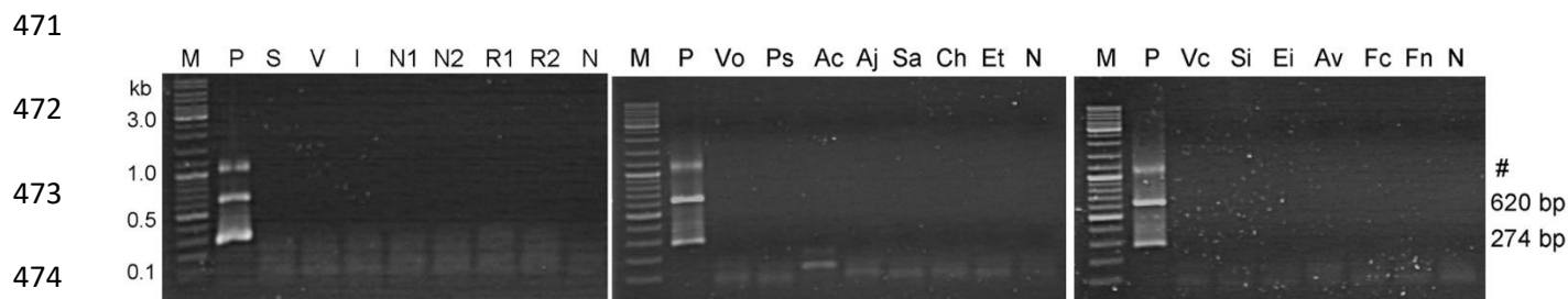
Figure S2 Specificity of the semi-nested TiLV detection assays. M, 2-log DNA marker (New England Biolabs); P, positive control using RNA extracted from TiLV-infected fish tissue as template; N, no template control; S, Scale Drop Disease Virus (SDDV); V, Nervous Necrosis Virus (NNV); I, Infectious Spleen and Kidney Necrosis Virus (ISKNV); N1/N2, clinically healthy Nile tilapia; R1/R2, clinically healthy red tilapia; Vo, Vogesella sp.; Ps, Pleisiomonas shigelloides ; Ac, Aeromonas caviae ; Aj, Aeromonas jandaei ; Sa, Streptococcus agalactiae ; Ch, Chryseobacterium sp.; Et, Edwardsiella tarda ; Vc, Vibrio cholerae ; Si, Streptococcus iniae ; Ei, E. ictaluri ; Av, Aeromonas veronii ; Fc, Flavobacterium columnare ; Fn, Francisella noatunensis subsp. orientalis . Details of bacterial isolates are shown in Table 2.
