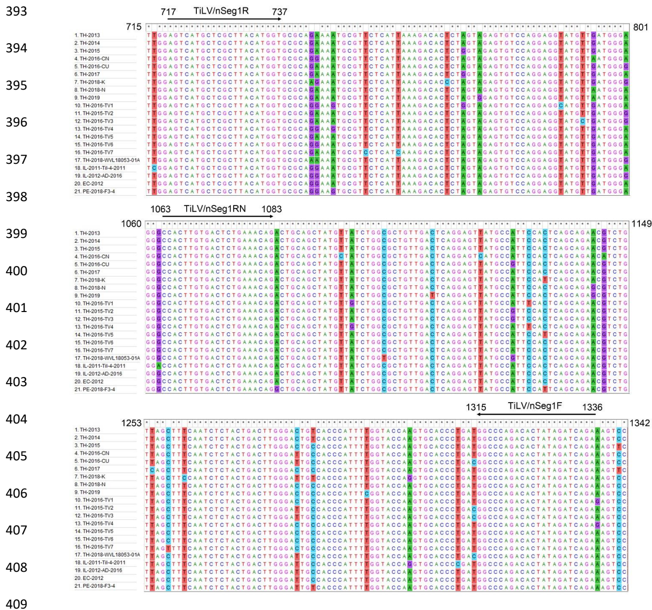
Figure 2 Multiple nucleotide sequence alignments of TiLV segment 1 PB1 genes of 21 viral isolates. A partial portion of an alignment is shown. Numbers represent nucleotide positions of the coding strand in the putative PB1 ORF. Arrows indicate sites that were used to design primers for the semi-nested RT-PCR protocol developed in this study. * marks nucleotide identity. Columns with differences in colors indicate nucleotide variability.
