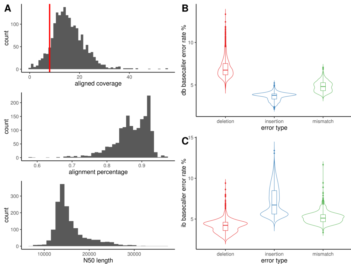
Fig. 1 Oxford Nanopore Technologies (ONT) long-read sequencing statistics. (A) Per individual distributions of aligned coverage (n = 1817, red vertical line denotes 8x coverage), aligned basepairs percentage, and N50 length (n = 1656, data from individuals with aligned coverage < 8x omitted). (B, C) Error rates compared to GRCh38 43 using deletion biased (db), and insertion biased (ib) basecallers, respectively, stratified by error type. Statistics are computed over all sequenced reads longer than 3000bp.
