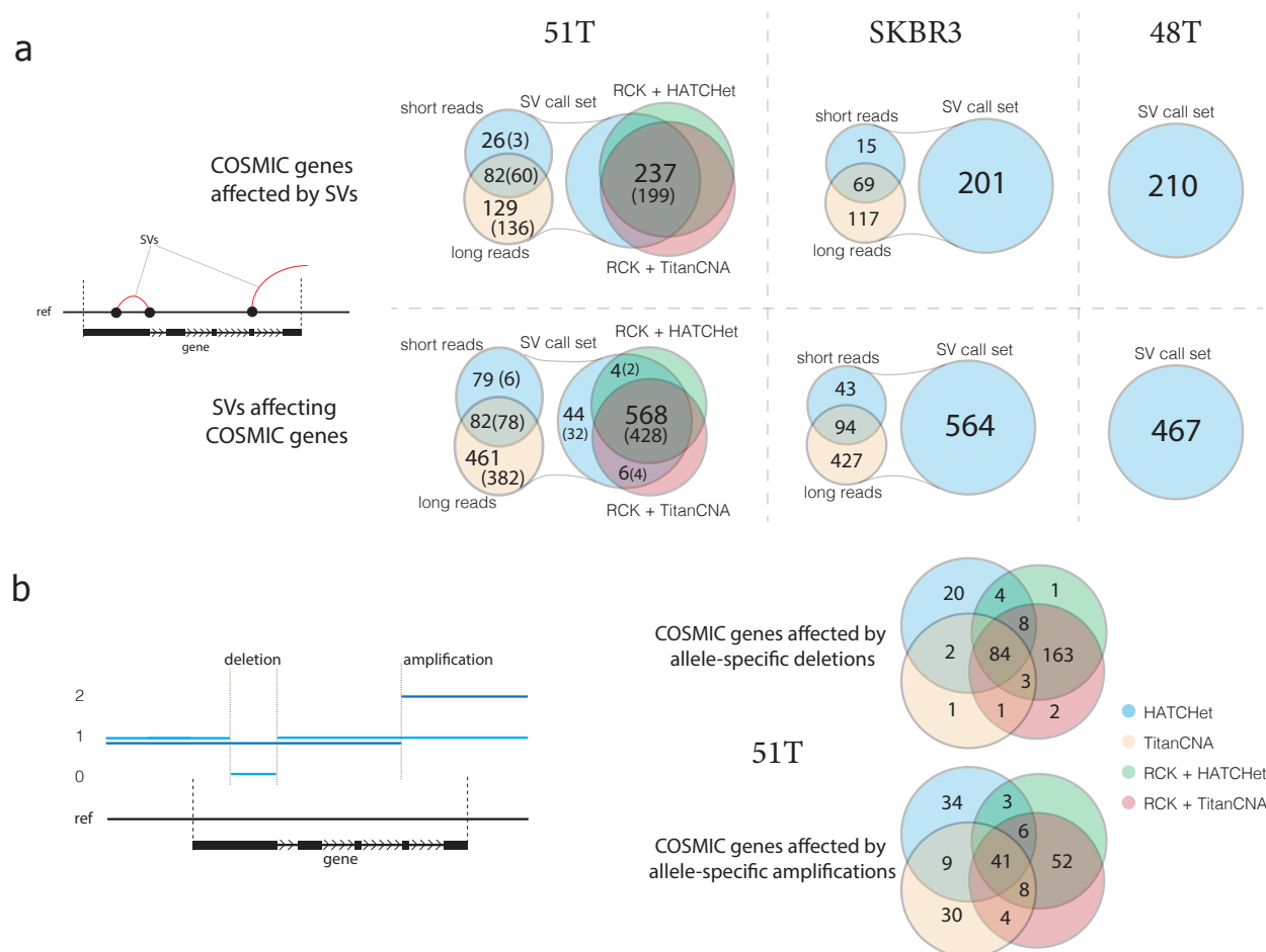
Figure 5. | Structural and Copy Number Variants in COSMIC census genes. a) Comparison of the the number of COSMIC census genes being affected by SVs, as well as the number of SVs affecting COSMIC census genes, across inferred SV callset in 51T and N (parenthetical), SKBR3, and 48T, and SVs reported by RCK as being present in the karyotypes reconstructed with either HATCHet or TitanCNA copy number profiles in 51T. b) Comparison of the number of COSMIC census genes affected by either allele-specific deletions or amplifications between copy number profiles from HATCHet, RCK+HATCHet, TitanCNA, and RCK+TitanCNA in 51T.
