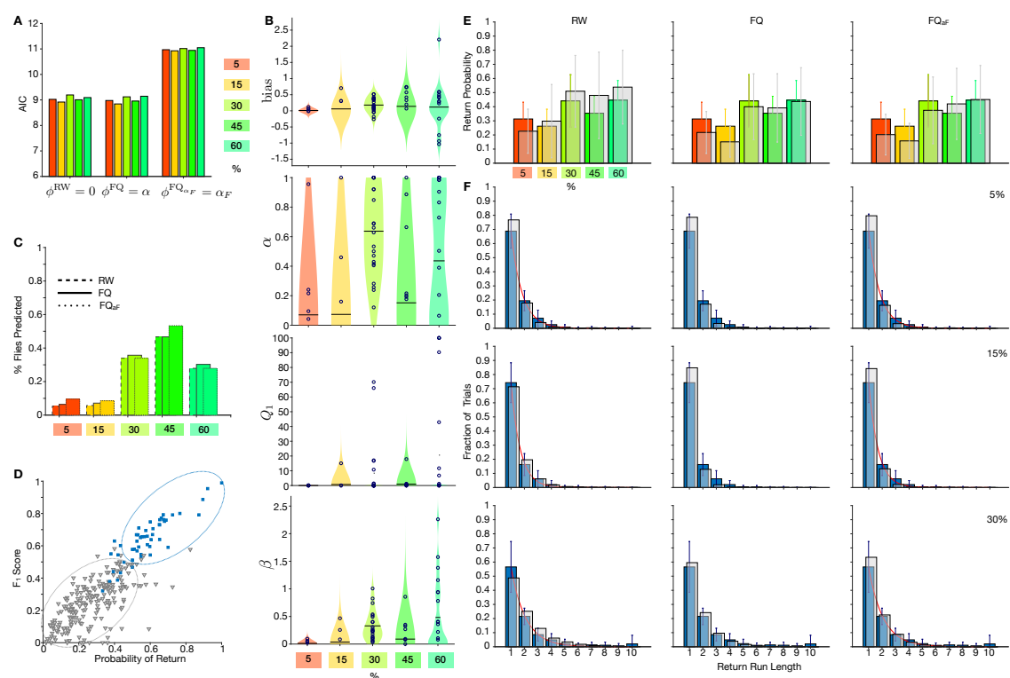
Figure S5: Reinforcement learning model selection, predictive test and generative test.
