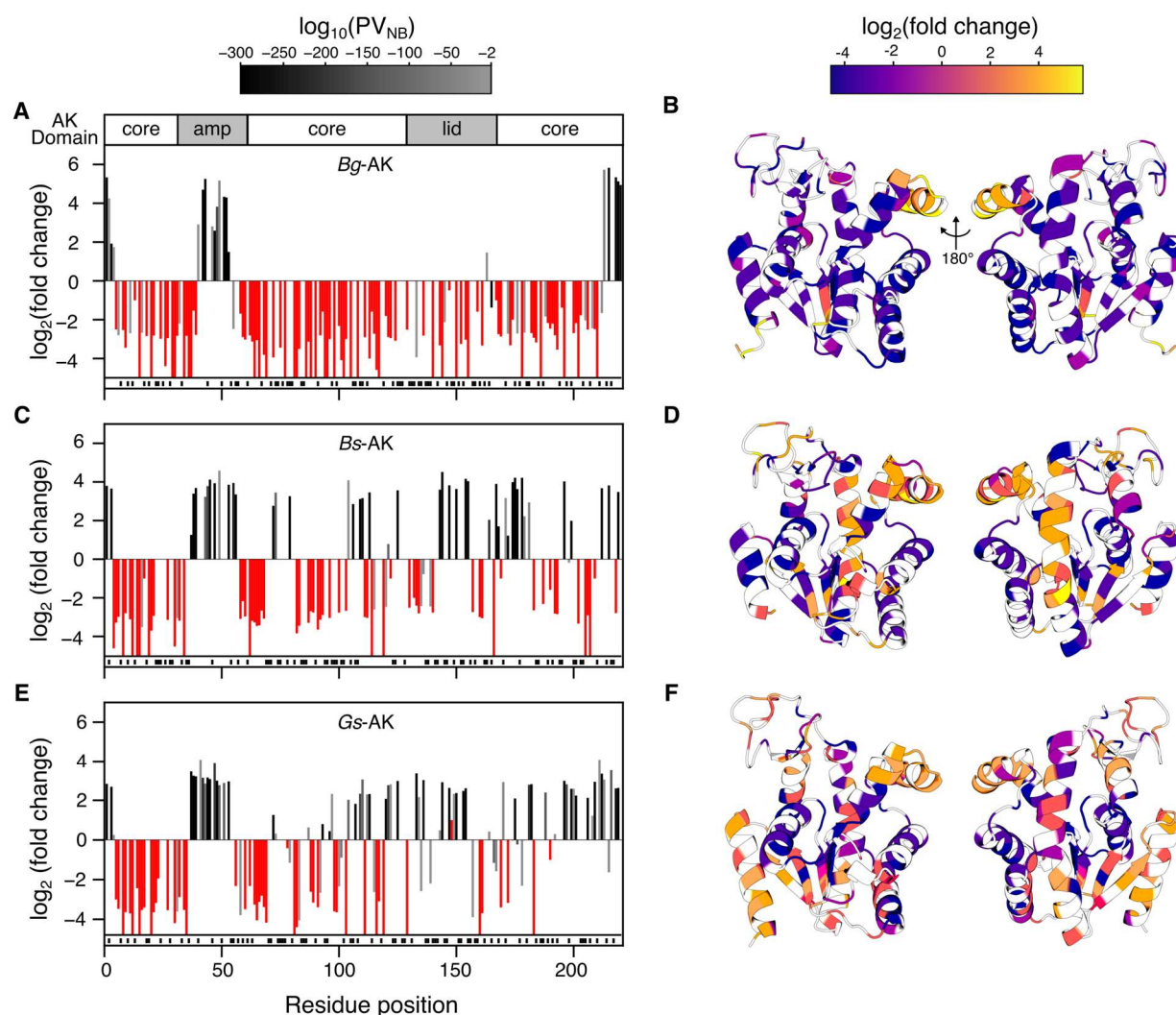
Figure 3. Comparison of circular permutation profiles of each AK. For each P variant, the \log_2(\text{fold change}) is shown as a function of the AK residue found at the N-terminus of the circularly permuted protein derived from (A) Bg-AK, (C) Bs-AK, and (E) Gs-AK. P -values obtained from the negative binomial model ( PV_{NB} ) are color coded with values >10^{-2} in red and variants having values \leq 10^{-300} in black and those variants displaying intermediate values shaded as indicated by the bar. The AK domain structure is shown at the top as a frame of reference. Variants no longer observed following selection are shown as bars that reach the line at the bottom of the graph. The cognate P and AP variant pairs absent from both the unselected and selected libraries ( n = 73, 72 , and 76 for Bg-AK, Bs-AK, and Gs-AK, respectively) are indicated as black lines shown below the x-axis. The \log_2(\text{fold change}) is compared with AK structure for (B) Bg-AK (PDB: 1S3G), (D) Bs-AK (PDB: 1P3J), and (F) Gs-AK (PDB: 1ZIO) with the residues colored according to their \log_2(\text{fold change}) as indicated by the bar. Unsampld positions are in white.
