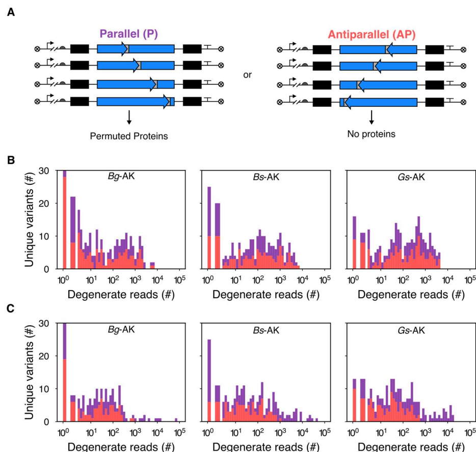
Figure 1. Permuted gene abundances versus gene orientation. (A) Generation of libraries using PERMUTE requires mixing a circular gene, a permuteposon, and MuA transposase. The permuteposon inserts in two orientations with equal frequencies (28). The orientation where the regulatory elements i.e. , promoter, RBS, and terminator, and the permuted genes are in the same direction is designated as parallel . Conversely, when the permuteposon inserts in the opposite direction such that the regulatory elements and the permuted genes are oriented in opposite directions this is designated as antiparallel . Only when the permuteposon inserts in the parallel orientation does it generate a vector capable of expressing a circularly permuted protein with an 18-residue peptide amended to the new N-terminus. For each (B) unselected library and (C) selected library we evaluated the number of degenerate, in-frame sequences at each position in both the P (purple) and AP (red) orientations.
