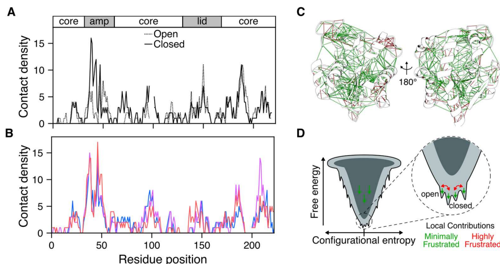
Figure 5. Energetic frustration of intramolecular contacts in adenylate kinase. (A) Frustratograms showing the calculated configurational frustration of the open (dashed) and closed (solid) conformations of Ec -AK (calculated from PDB: 4AKE and 1AKE, respectively). The density of contacts in a 5Å sphere with highly frustrated contact energies is plotted at every AK residue position. (B) A comparison of the frustratograms of the closed conformations of Bg -AK (blue), Bs -AK (purple), and Gs -AK (red). (C) The contact energy frustration is mapped onto the tertiary structure of a closed structure (PDB: 1AKE). Highly frustrated contacts are displayed in red, while minimally frustrated are shown in green. Direct contacts are solid lines, while water mediated contacts are dashed lines. (D) Influence of contact frustration on the global protein folding and functional energy landscape. Minimally frustrated contacts promote protein folding into the low-energy native ensemble, while within this ensemble highly frustrated contacts facilitate the sampling of conformations including those important for catalysis.
