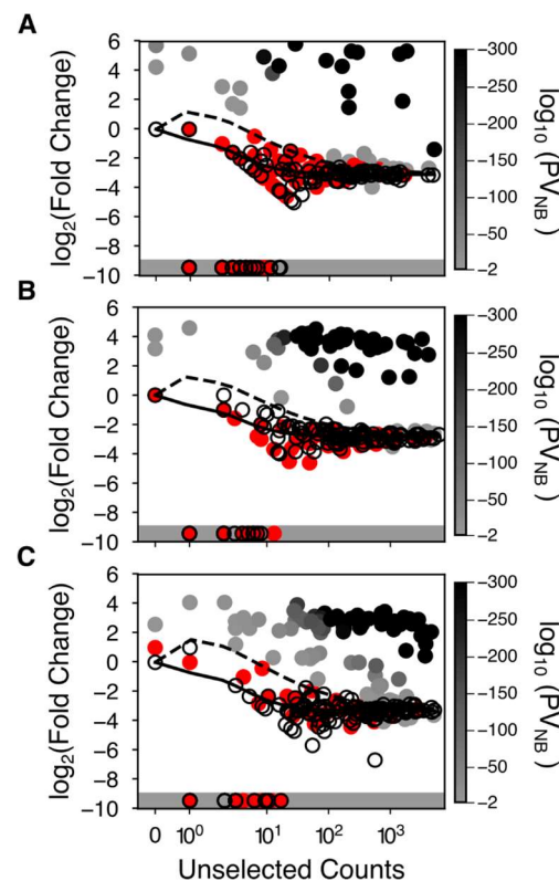
Figure S3. Fold enrichment as a function of the initial abundance and statistical model. The \log_2(\text{fold change}) in sequence abundances of the AP (open symbols) and P variants (closed symbols) for (A) Bg -AK, (B) Bs -AK, and (C) Gs -AK. The significance of P variant enrichment obtained using the negative binomial model ( PV_{NB} ) is colored as a function of the P -value obtained with the variants presenting values >0.01 in red, variants having values \leq 10^{-300} in black and those variants displaying intermediate values shaded as indicated in the bar. The black line represents the mean dilution for AP variants relative to their initial abundance in the unselected library, while the dashed line represents two standard deviations greater than the mean. Variants not observed in the selected library (infinitely diluted) are plotted in the shaded region.
