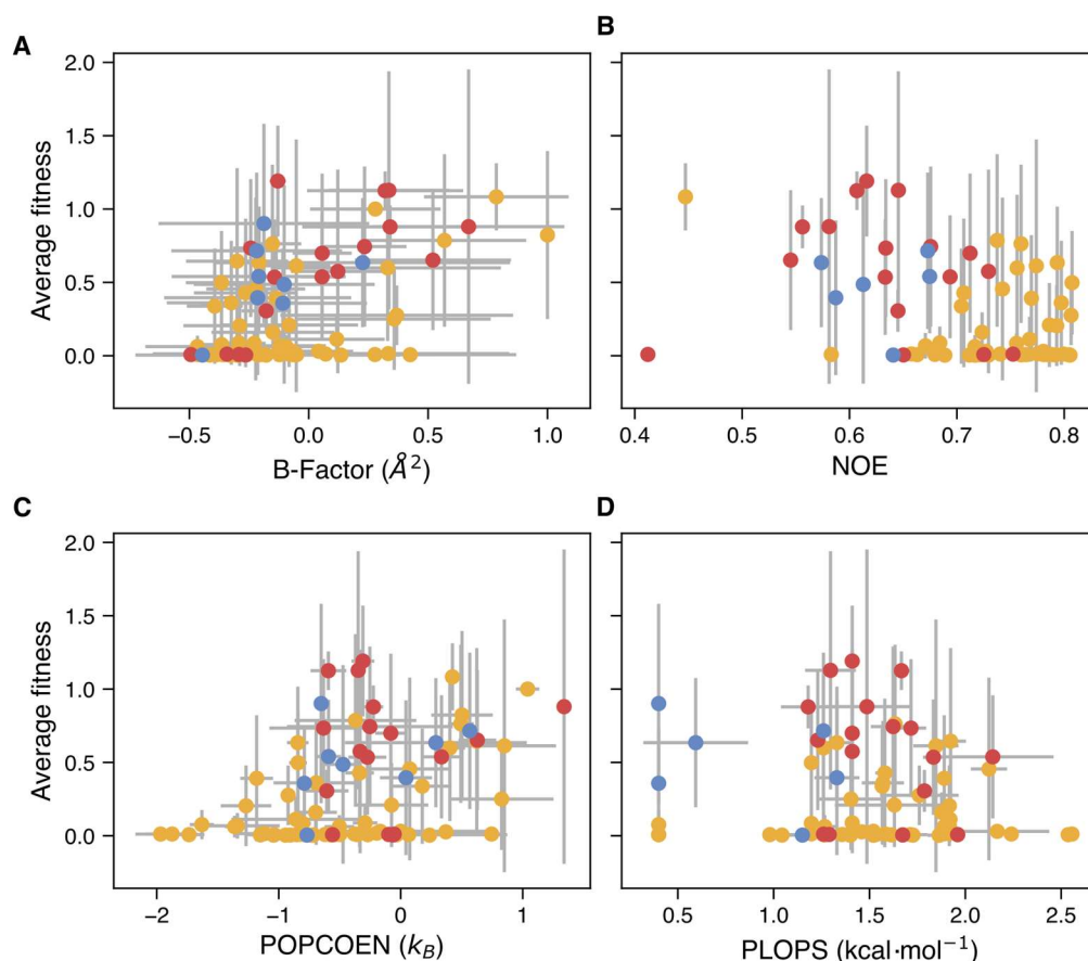
Figure S6. Comparison of protein dynamics metrics with the average fitness of permuted proteins. The average fitness (fold change relative to native AK) of each trio of orthologous permuted proteins is compared to (A) the average normalized B-factors from each crystal structure ( R_{SR}=0.439 , P -value = 2.95 \times 10^{-5} ), (B) the NOE data from Ec -AK (2) ( R_{SR}=-0.324 , P -value = 6.00 \times 10^{-3} ), (C) predictions of residue-level conformational entropy resulting from POPCOEN (3) ( R_{SR}=0.380 , P -value = 3.71 \times 10^{-4} ), and (D) prediction of residue-level conformational entropy loss upon folding resulting from PLOPS (4) ( R_{SR}=0.015 , P -value = 8.96 \times 10^{-1} ). B-factors were normalized using a previously described method (5)
