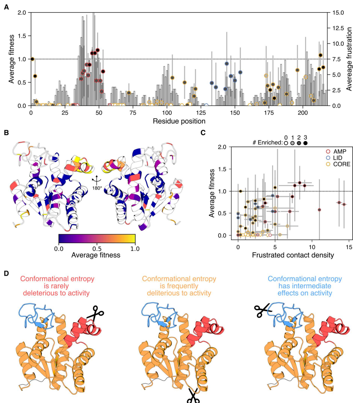
Figure 6. Comparison of family permutation profiles and energetic frustration. (A) For topological mutants that were sampled in all three libraries ( n = 84 ), the average fitness and average frustration are compared to the position in the primary structure. The circles represent the average fitness of each variant with the standard deviation shown in gray. The shading of each circular data symbol represents the number of orthologs in which the variant was found to be enriched. The bars represent the average density of highly frustrated contacts at each position observed across all three structures. The dotted line represents the native AK fitness. (B) The average fitness of all three orthologs is compared to the tertiary structure (PDB: 1S3G). The color of the residue corresponds
