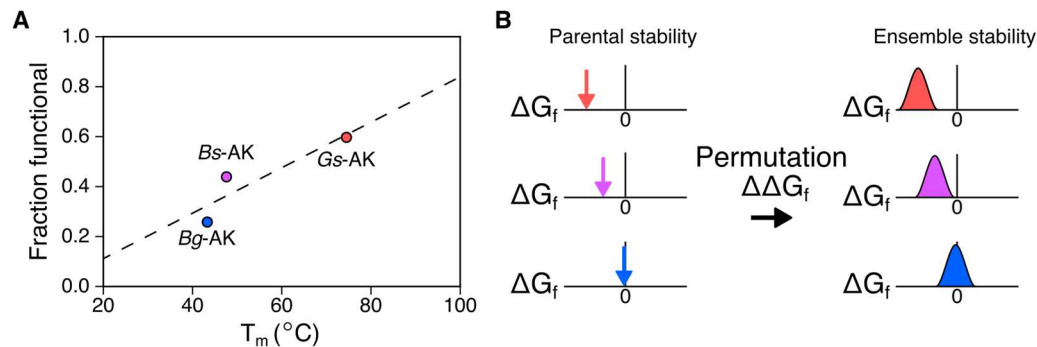
Figure 2. Thermodynamic stability correlates with tolerance to permutation. (A) The fraction of P variants sampled in the libraries that were biologically active following selection is plotted relative to the melting temperature of each AK parent. A linear fit ( y = 0.01x - 0.07 , R^2 = 0.822 ) is shown as a dashed line. (B) This trend suggests that circular permutation has similar destabilizing effects on structurally-related AK homologs yielding a similar ensemble of \Delta\Delta G_f .
