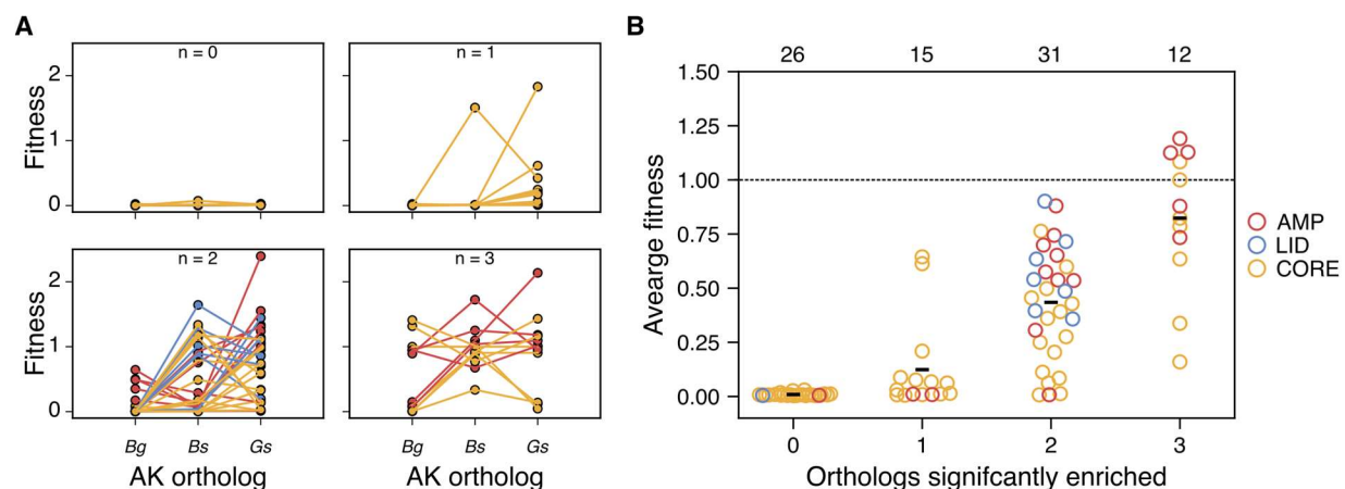
Figure 4. Comparison of family enrichment and fitness. (A) For variants that were sampled in all three AK libraries ( n = 84 ), the fitness score (fold change relative to native AK) is shown. In each box, the number of AK homologs across the three libraries that were found to be significantly enriched using PV_{NB} is noted as 0, 1, 2, or 3. Data for each topological variant is connected by a line to illustrate the trend across homologous permuted proteins derived from parent AKs having distinct thermostabilities. Those topological mutants that were uniformly biologically active across all three libraries ( n = 3 ) presented a wide range of fitness values (ranging from 0.004 to 2.13). (B) For the same set of circularly permuted protein homologs, the average fitness of all three orthologs is compared to the number of orthologs found to be significantly enriched using PV_{NB} . The number of data points in each bin is noted at the top. The average fitness of all the orthologs in a column is noted with the short black line, while the average fitness of the native AKs are indicated by the dashed line. The domain location of the new protein termini in each permuted protein trio is indicated by the color of the ring according to the legend.
