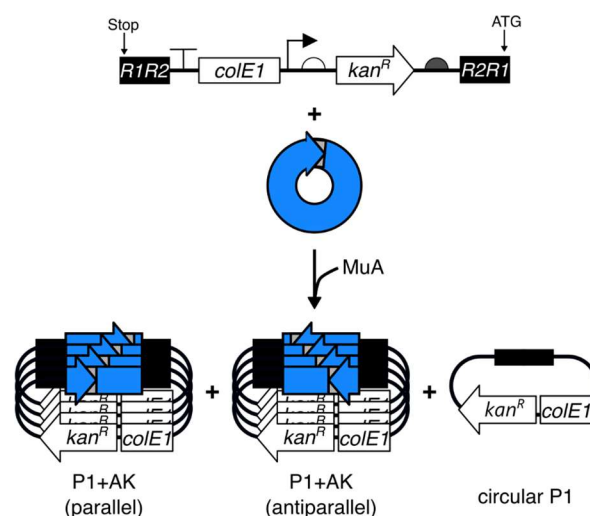
Figure S8. Analysis of permuted MuA libraries. (A) PERMUTE protocol uses MuA transposase to insert a permuteposon randomly into a circularized gene, which eliminates the need for using a target vector. The product of this reaction yields circularized permuteposon (P1) and the desired permuteposon + AK gene hybrids (P1 + AK) in both the parallel and antiparallel orientations.
