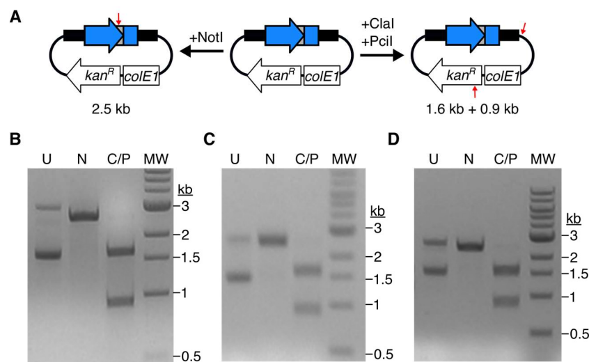
Figure S9. Size-selected permuted libraries are homogeneous for P1 + AK hybrids. (A) Following purification of the P1 + AK hybrids from the MuA libraries, the size-selected libraries were subjected to NotI (N) digests expected to yield a 2.5 kb fragment and Clal/PciI (C/P) double digests expected to yield 1.6 and 0.9 kb fragments. Restriction site locations are marked by red arrows. Agarose gel electrophoresis of the digests reveals the correct bands in (B) Bg -AK, (C) Bs -AK, (D) Gs -AK libraries compared to the uncut MuA library control (U).
