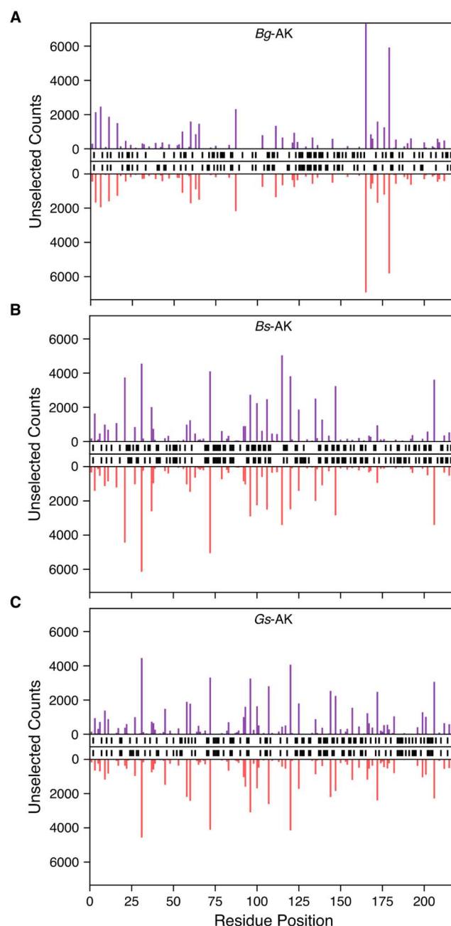
Figure S2. Sequence abundances as a function of the first AK codon in each ORF. A comparison of the AK codon at the beginning of each permuted gene and the number of P (purple) and AP (red) sequence reads observed in the unselected libraries for (A) Bg -AK, (B) Bs -AK, and (C) Gs -AK. In cases where a P or AP variant was absent, black bars are shown between the x-axes.
