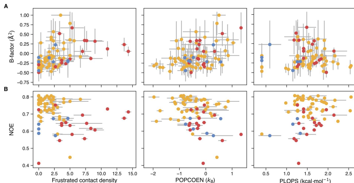
Figure S7. Comparison of experimental measures of protein dynamics with computational metrics. The pairwise comparison of (A) B-factors and (B) NOE data from Ec -AK is compared with predictions of the frustrated contact density calculated using the frustratometer, predictions of residue-level conformational entropy calculated using POPCOEN (3), and PLOPS predictions of residue-level conformational entropy loss upon folding (4). Correlations between the metrics are as follows: B-Factor and frustrated contact density ( R_{SR}=0.573 , P\text{-value} = 1.22 \times 10^{-8} ), B-factor and POPCOEN ( R_{SR}=0.348 , P\text{-value} = 1.18 \times 10^{-3} ), B-factor and PLOPS ( R_{SR}=0.073 , P\text{-value} = 5.24 \times 10^{-1} ), NOE and frustrated contact density ( R_{SR}=-0.315 , P\text{-value} = 7.95 \times 10^{-3} ), NOE and POPCOEN ( R_{SR}=-0.316 , P\text{-value} = 7.76 \times 10^{-3} ), and NOE and PLOPS ( R_{SR}=0.133 , P\text{-value} = 2.87 \times 10^{-1} )
