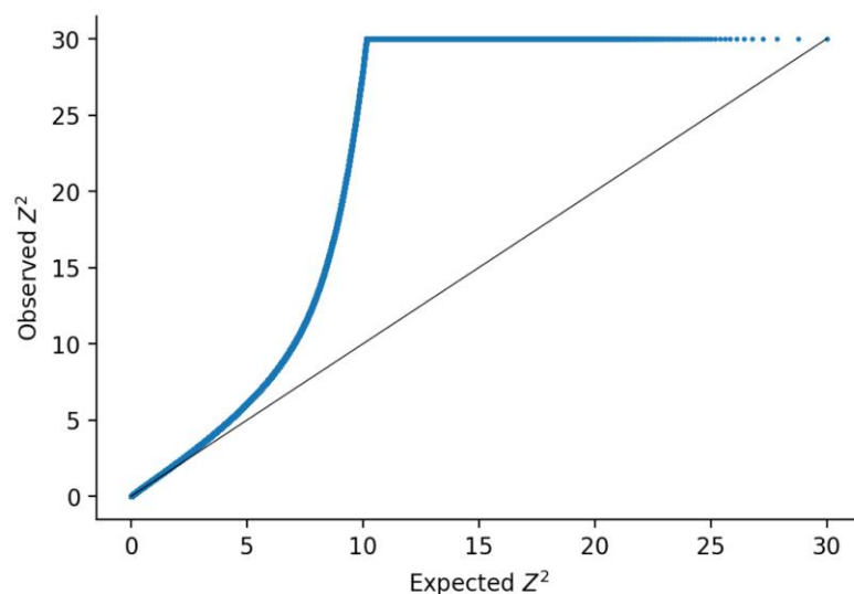
Supplementary Fig. S2: Quantile-quantile (QQ) plot of all associations in PhenomeXcan and ClinVar traits. The expected \chi^2 null distribution is plotted along the black diagonal, and the entire distribution of observed Z^2 is plotted in blue. We do not see evidence of systematic inflation given the initial consistency in expected and observed p-values. (To improve visualization, Z^2 are thresholded at 30.) The increase in the QQ plot for observed p-values can be seen with the extremely large number of associations tested (20.6 million) as well as the pleiotropy we identify with trait-trait associations in which multiple genes are involved. Z^2 correspondence to percentiles were as follows: 95th percentile: Z^2=4.45 , 99th percentile: Z^2=9.07 , 99.9th percentile: Z^2=214.45 . A Z^2 of 6 represents a Bonferroni-adjusted p-value of 0.05.
