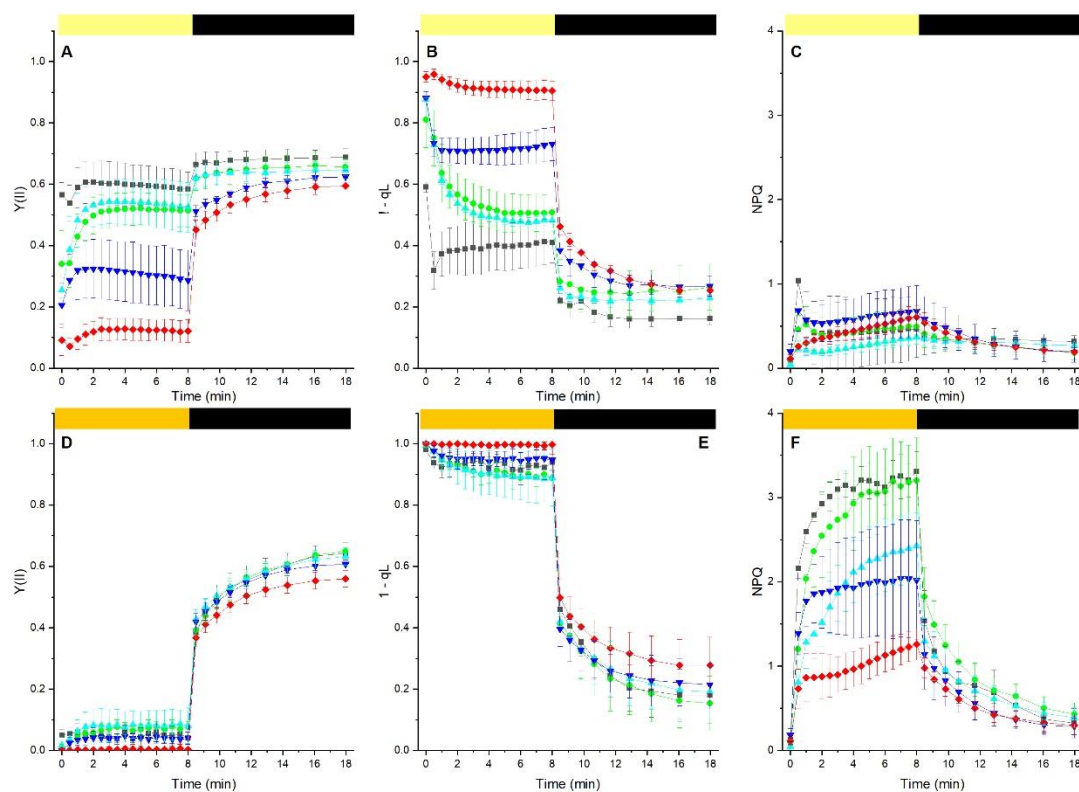
Figure S6. Photosystem II functionality under dim / High illumination. Yield of PSII (Y(II); A,D), PQ reox state (1-qL; B-E) and non-photochemical quenching (NPQ; C-F) were measured with Dual-PAM 100 under dim (50 \mu\text{mol photons m}^{-2}\text{s}^{-1} , A-C) or high (550 \mu\text{mol photons m}^{-2}\text{s}^{-1} , D-F) illumination. Actinic light (upper yellow bar) was switched off after 8 min. In all panels WT is shown in black, flva-pgrl1 in cyan, flva-ndhm in green, pgrl1-ndhm in blue and flva-pgrl1-ndhm in red. Data are shown as average \pm SD (n > 4).
