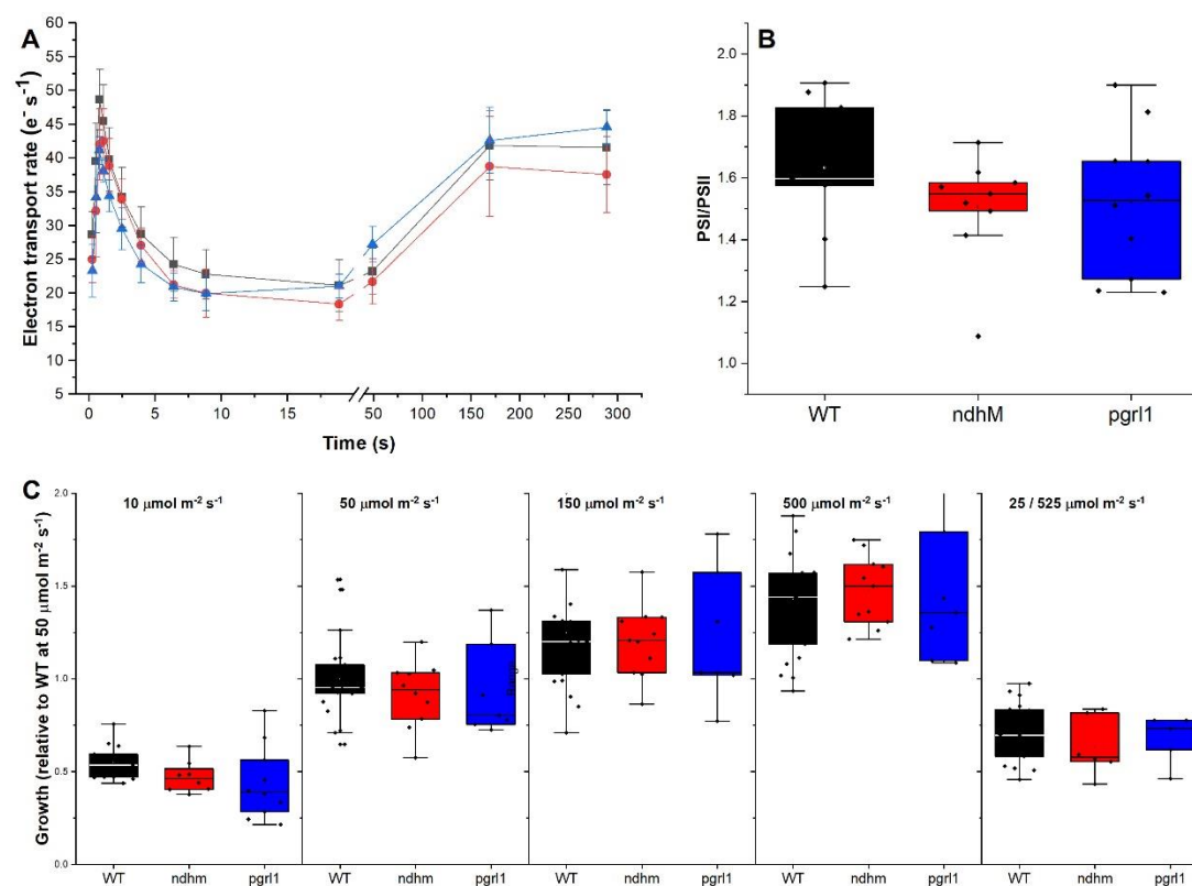
Figure S2. Phenotype of pgrl1 and ndhm KO. A) Electron transport rate, calculated from electrochromic shift, of dark acclimated plants after illumination with saturating light ( 940 \mu mol photons m^{-2} s^{-1} ) for 300s. Electron transport was normalized to total charge separation capacity (thus to the activity of both PSI and PSII) quantified from single turnover pulse excitation. Data are represented as mean and standard deviation is also reported ( n > 10 ). B) PSI/PSII ratio calculated from single pulse excitation. PSI contribution was measured in presence of DCMU that inhibits PSII activity. C) Quantification of the growth of P. patens WT and pgrl1 and ndhm KO grown under illumination of different intensity: limiting (LL, 10 \mu mol photons m^{-2} s^{-1} ), optimal (CL, 50 \mu mol photons m^{-2} s^{-1} ), excess light (ML and HL, 150 and 500 \mu mol photons m^{-2} s^{-1} ); or light fluctuations (FL, 3 minutes at 525 \mu mol photons m^{-2} s^{-1} and 9 minutes at 25 \mu mol photons m^{-2} s^{-1} ). In B and C, plots depict median and 25-75 percentiles as boxes, minimum and maximum values as whiskers and outliers as external points, individual data points are also superimposed to the boxes. In all panels WT is shown in black, ndhm in red and pgrl1 in blue.
