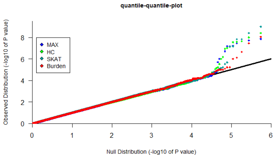
Figure 4. Real data analysis of 897 asthmatic offspring trios in a WGS study. Quantile-quantile plot for Burden, SKAT, MAX, and HC test statistics based on approximately 547,000 windows of 50 consecutive rare variants.
