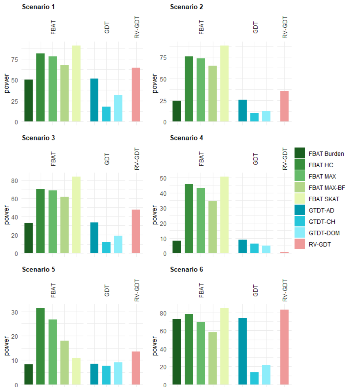
Figure 2. Power results in six different scenarios for genetic regions consisting of 50 variants at a significance level of \alpha = 0.05 . All results based on 1,000 replicates.
