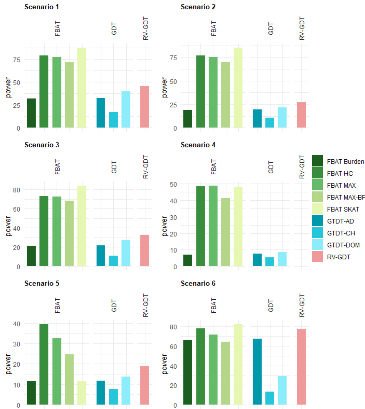
Figure 1. Power results in six different scenarios for genetic regions consisting of 30 variants at a significance level of \alpha = 0.05 . All results based on 1,000 replicates.
