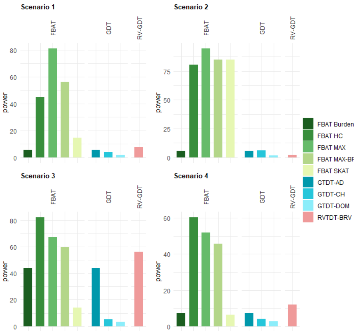
Figure 3. Power results for four different scenarios for genetic regions consisting of 1,000 variants at a significance level of \alpha = 0.05 . All results based on 1,000 replicates.
