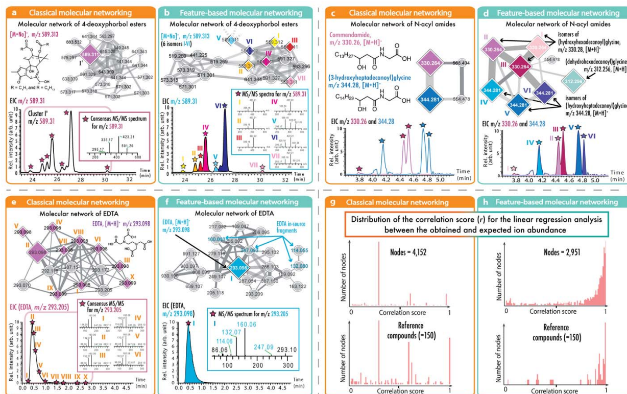
Fig. 2: Comparisons of classical MN and feature-based molecular networking. In these examples, the node size corresponds to the spectral count in classical MN (orange boxes, left) or to the sum of LC-MS peak area in FBMN (blue boxes, right). Panel (a) displays the results from classical MN with the LC-MS 2 data of Euphorbia dendroides plant samples; classical MN resulted in one node for the ion at m/z 589.313, while (b) FBMN performed after MZmine processing was able to detect seven isomers of this ion. Classical MN in the data of a cohort from the American Gut Project (c) showed two different N -acyl amides while the use of FBMN (d) processed with MZmine allowed the annotation of three different isomers per N -acyl amides. Classical MN (e) and FBMN (f) performed with OpenMS, were used to analyse the network of EDTA in plasma (373 samples) by compressing MS 2 spectra of EDTA eluting over 2.5 min into one best-quality MS 2 spectrum. FBMN recovered the molecular similarity of in-source fragments observed for EDTA, which were not displayed with classical MN, due to the fixed top-K rank for connected nodes (typically set to 10) of MS 2 spectral similarity. Evaluation of quantitative performance using a serial dilution of serum reference sample (NIST1950SRM) analyzed with (g) classical MN and (h) FBMN. The plots are showing the correlation score ( r ) distribution between the observed and expected relative ion abundance. The upper charts present the distribution of the correlation score for all the nodes (features) generated, and the bottom charts show the distribution for 150 reference compounds. While classical MN uses the spectral count or the sum precursor ion count to estimate the molecular network node abundance, FBMN uses the LC-MS feature abundance (peak area or peak height), resulting in a more accurate estimation of the relative ion intensity.
