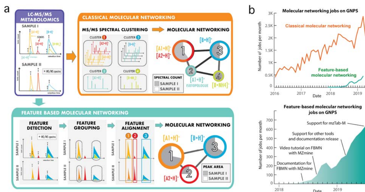
Fig. 1: Methods for the generation of molecular networks from non-targeted mass spectrometry data with the GNPS web platform. a) Two methods exist for the generation of molecular networks on the GNPS web platform: classical MN and feature-based molecular networking (FBMN). For both methods, mass spectrometry data files have to be converted to the mzML format using tools such as Proteowizard MSConvert 25 . The classical MN method runs entirely on the GNPS platform. In that method, MS 2 spectra are clustered with MS-Cluster and the consensus MS 2 spectra obtained are used for classical MN generation. In the case of FBMN, a feature detection and alignment tool is used to first process the LC-MS 2 data (such as MZmine, MS-DIAL, XCMS, OpenMS, Progenesis QI, or MetaboScape) instead of using MS-Cluster (classical MN). Results are then exported and uploaded to the GNPS web platform for molecular networking analysis. b) Graphs showing the number of molecular networking jobs performed on GNPS. The upper graph shows the number of classical MN and FBMN jobs since 2016. The lower graph shows the number of FBMN jobs since its introduction in 2017 and key events accelerating its use.
