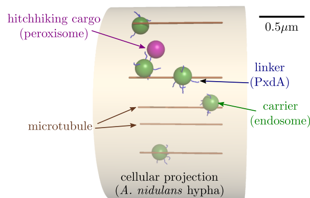
Figure 1: Schematic of the model for hitch-hiking initiation. A simulation snapshot is shown with all model components labeled. Specific components for peroxisome hitchhiking in Aspergillus nidulans are indicated in parentheses. Scale bar: 0.5 \mu\text{m} .
