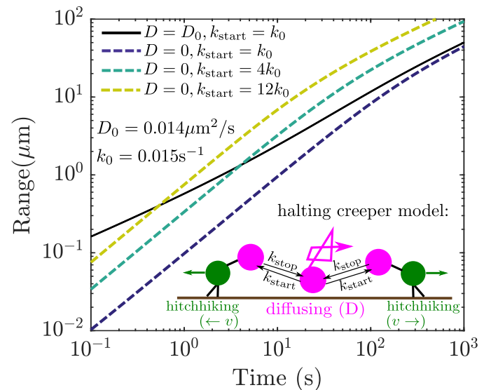
Figure 6: Range of a halting creeper particle engaged in bidirectional runs alternating with diffusive or tethered periods. Solid black line gives range for a particle that diffuses freely with diffusivity D_0 , between processive runs initiated with a rate k_0 . Dashed lines give range for particles that are tethered when not engaged in an active run, but with increasing initiation rates.
