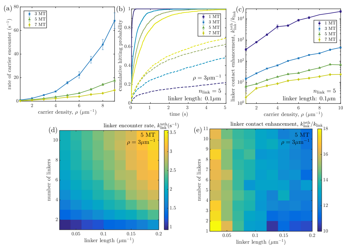
Figure 5: Effect of cargo tethering to microtubule on encounter rates with carrier organelles and their linker proteins. (a) Rate of encounter with a carrier organelle, for different numbers of microtubules in the domain. (b) Cumulative hitting probability with the tip of a linker protein, for tethered (solid lines) and untethered cargo (dashed lines), showing more rapid encounters in the tethered case. (c) Enhancement of overall contact rate with a linker protein tip, due to tethering of cargo. (d) Encounter rate between a tethered cargo and linker protein tip, as a function of linker length and number. (e) Ratio of encounter rates with linker protein tips, for a tethered versus diffusive cargo.
