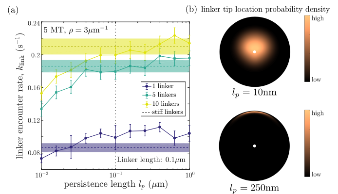
Figure 4: Dependence of encounter rate on linker flexibility. (a) Rate at which cargo encounters a linker tip, as a function of linker persistence length for different linker numbers. Dashed lines with shaded areas denote contact rate for infinitely stiff linkers along with standard error. Dotted vertical line denotes \ell_p = 0.1\mu\text{m} , used in all other simulations. (b) End distribution of a WLC of length \ell = 100\text{nm} with initial orientation fixed, highlighting the increased extension \Delta z yet smaller area coverage of stiffer linkers. Top: \ell_p = 10\text{nm} , bottom: \ell_p = 250\text{nm}
