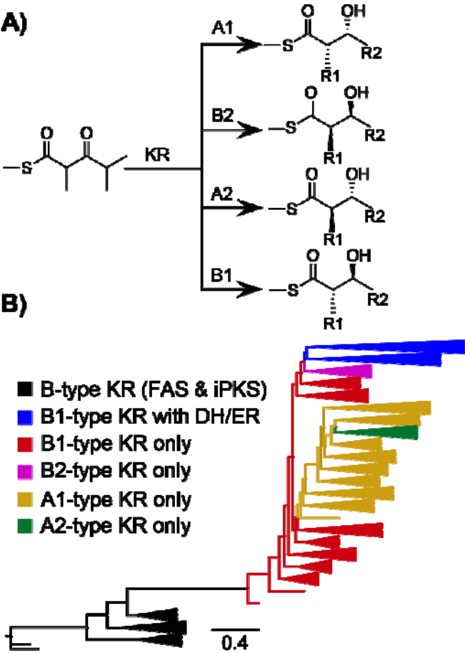
Figure 1. Bioinformatic analysis of reductive loop exchanges. A) KR subtypes determine the stereochemistry of the \beta -hydroxyl and \alpha -carbon B) Phylogenetic tree of the ketoreductase (KR) domain of all manually curated KRs in ClusterCAD determined by ModelFinder in IQ-Tree.
