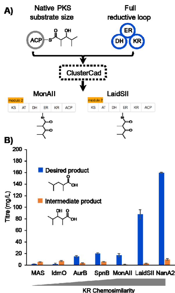
Figure 3. A chemoinformatic approach to reductive loop exchanges. A) A search in ClusterCad revealed the closest substrates to the first module of lipomycin containing a full reductive loop B) Production levels of reductive loop exchanges with the closest KR substrate similarity to LipPKS1 (MonAII, LaidSII and NanA2) compared to donor loops with less KR substrate similarity (MAS, IdmO, AurB, SpnB).
