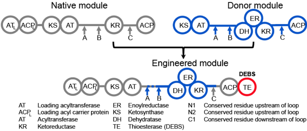
Scheme 1. Experimental design of PKS reductive loop swaps. Conserved residues are identified through multiple sequence alignment surrounding the reductive domains (“A”, “B” and “C”). Donor reductive loops are inserted into the native lipomycin module, and the DEBS thioesterase cleaves the product.
