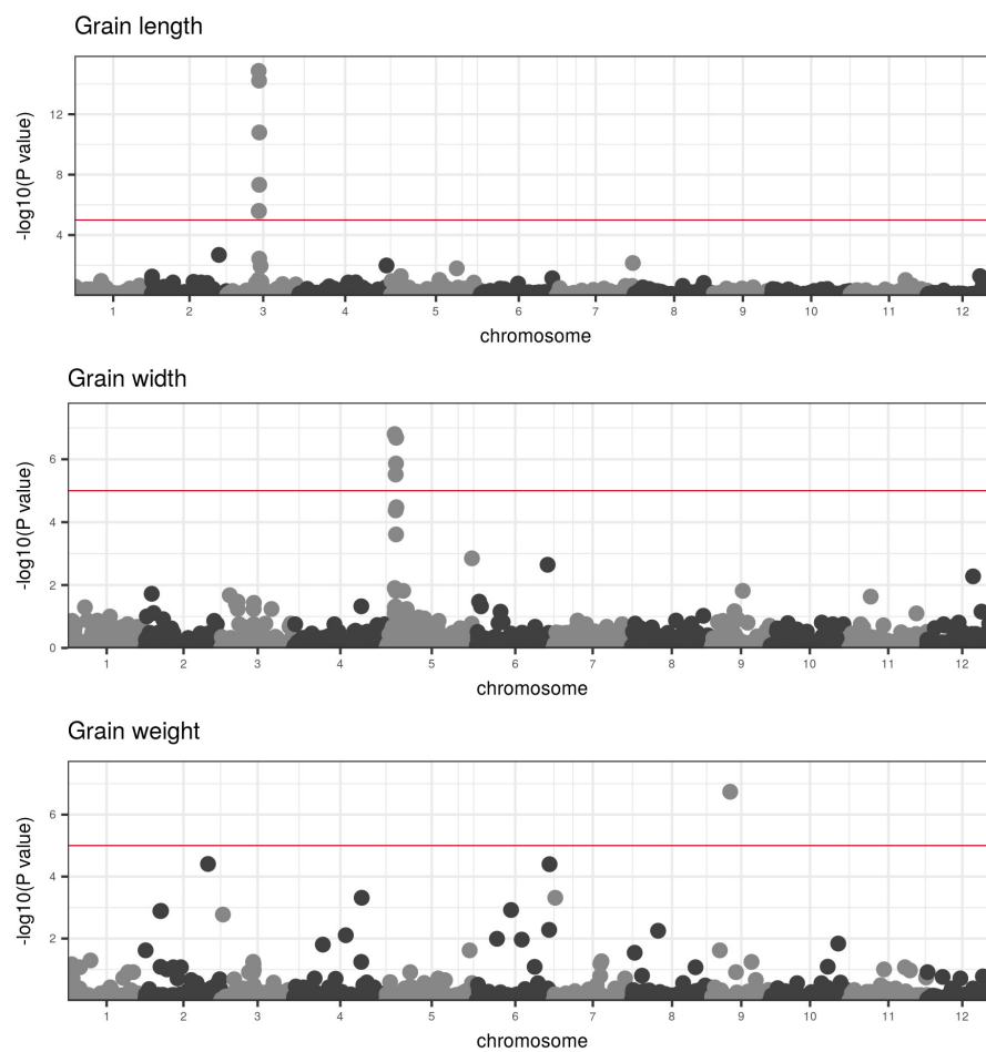
Figure 2: Manhattan plots for grain length, grain width and grain weight after false discovery rate correction at a significance level of -\log_{10}(1e-5) .
