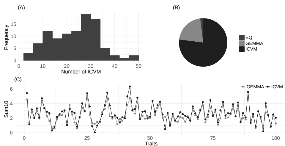
Figure 3: Graphical representations of the results from the simulation experiments. (A) shows the distribution of the number of markers selected using the proposed approach. (B) shows the proportion of the simulated traits for which GEMMA and ICVM performed best on Sum10 analysis. Eq is the proportion for which GEMMA and ICVM performed equally. (C) shows the Sum10 values for GEMMA and ICVM on the simulated traits.
