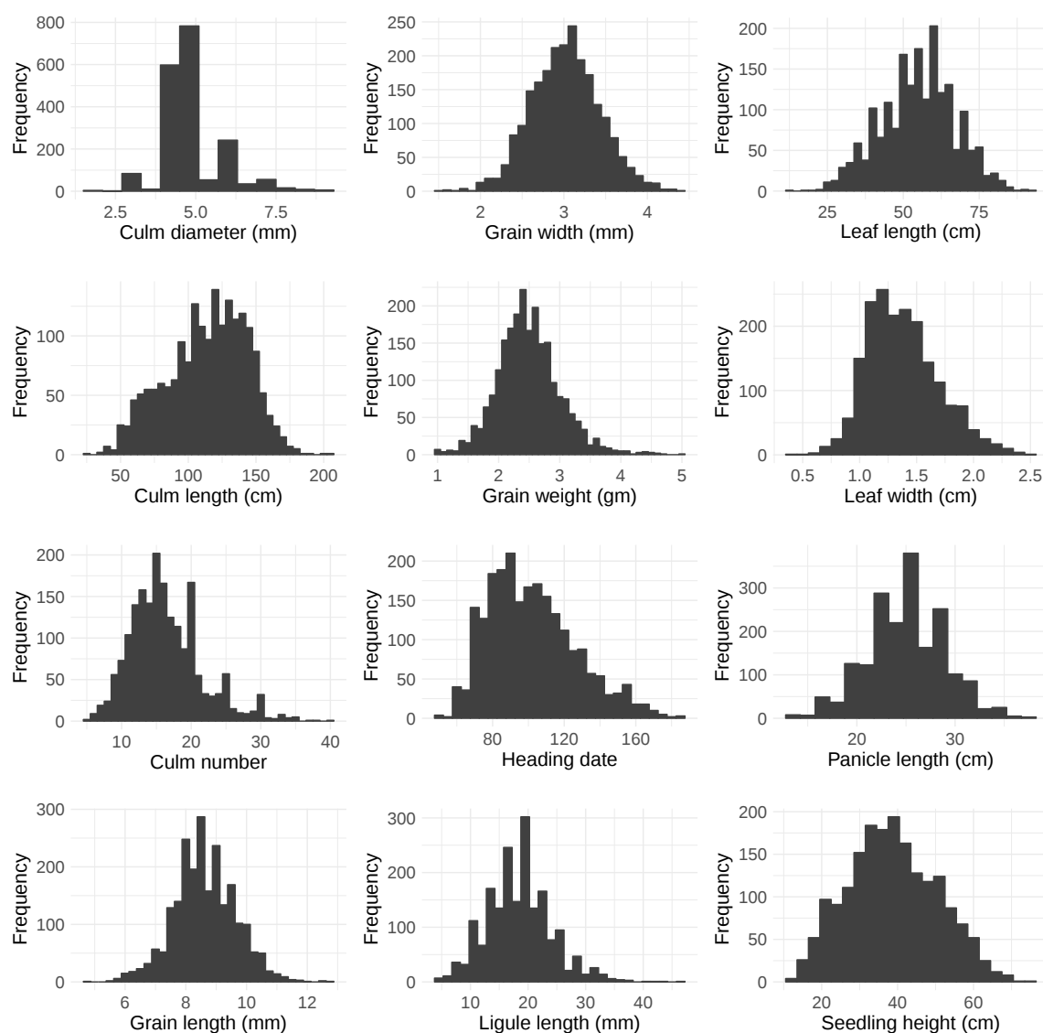
Figure 4: Distribution of traits used in this study.
