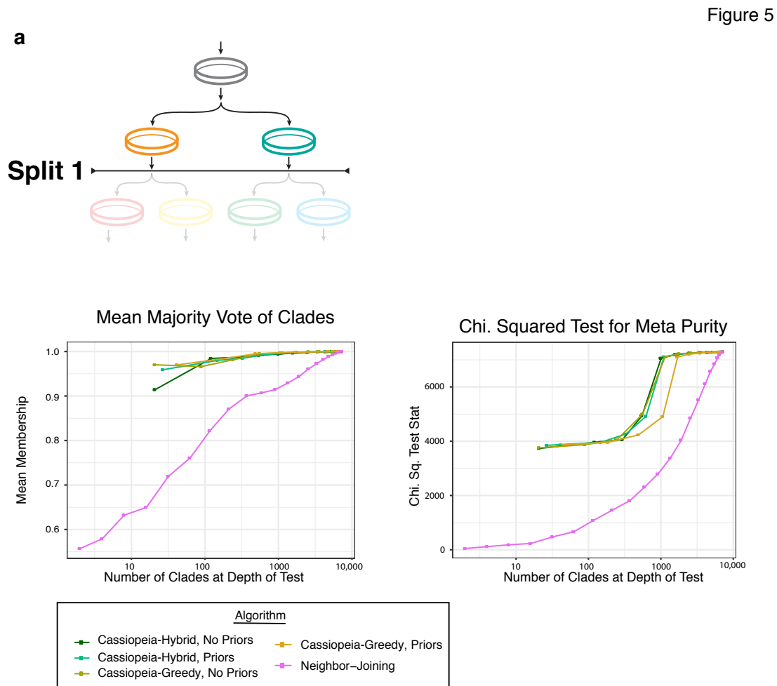
Figure 5: Cassiopeia builds highly accurate trees from large empirical datasets.
