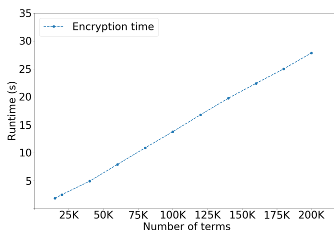
Figure S7: Run time needed for encrypting an increasing number of clinical attributes and genetic variants at a data provider computer (before upload to the system).
