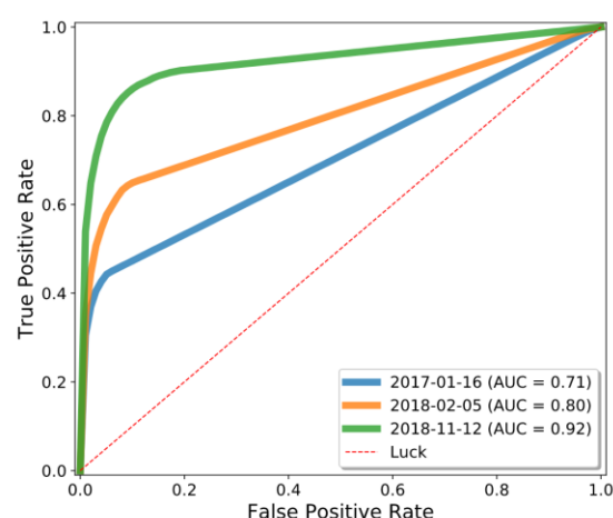
Figure 5. Drug repurposing using the Wikidata knowledge graph. We analyzed three snapshots of Wikidata using Rephetio, a graph-based algorithm for predicting drug repurposing candidates [63]. We evaluated the performance of the Rephetio algorithm on three historical versions of the Wikidata knowledge graph, quantified based on the area under the receiver operator characteristic curve (AUC). This analysis demonstrated that the performance of Rephetio in drug repurposing improved over time based only on improvements to the underlying knowledge graph. Details of this analysis can be found at https://github.com/SuLab/WD-rephetio-analysis .
