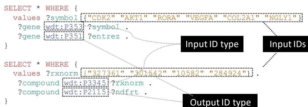
Figure 2. Generalizable SPARQL template for identifier translation. This simple example shows how identifiers of any biological type can easily be translated using SPARQL queries. These queries operate on Wikidata properties for gene symbols (wdt:P353) and Entrez Gene IDs (wdt:P351) (top), and RxNorm concept IDs (wdt:P3345) and NDF-RT IDs (wdt:P2115) (bottom). These queries can be submitted to the Wikidata Query Service (WDQS; https://query.wikidata.org/ ) to get real-time results from Wikidata data. Relatively simple extensions of these queries can also be added to filter mappings based on the statement references and/or qualifiers. A full list of Wikidata properties can be found at [43]. Note that for translating a large number of identifiers, it is often more efficient to perform a SPARQL query to retrieve all mappings and then perform additional filtering locally.
