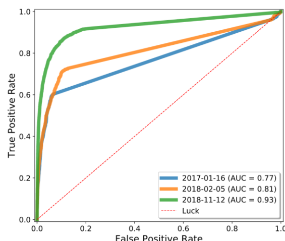
Supplemental Figure 1. Drug repurposing using the Wikidata knowledge graph, evaluated using an external test set.
