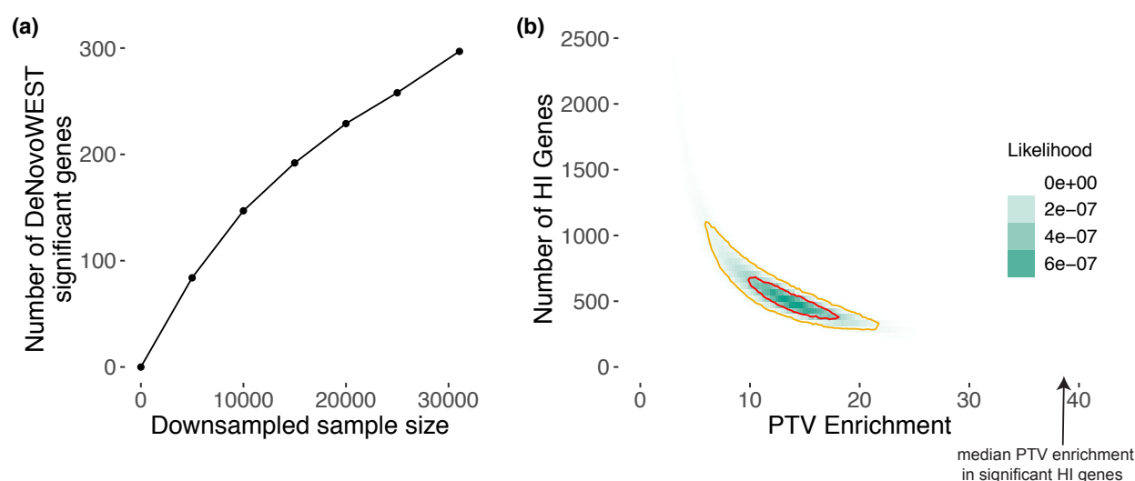
Figure 4: Exploring the remaining number of DD genes. (a) Number of significant genes from downsampling full cohort and running DeNovoWEST's enrichment test. (b) Results from modelling the likelihood of the observed distribution of de novo PTV mutations. This model varies the numbers of remaining haploinsufficient (HI) DD genes and PTV enrichment in those remaining genes. The 50% credible interval is shown in red and the 90% credible interval is shown in orange. Note that the median PTV enrichment in significant HI genes (shown with an arrow) is 38.8.
