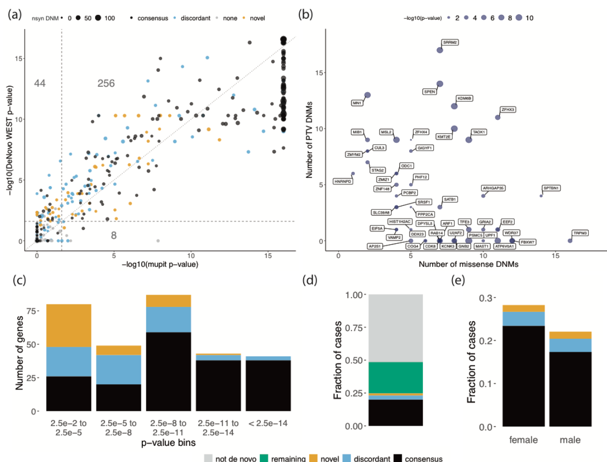
Figure 1: Results of DeNovoWEST analysis. (a) Comparison of p-values generated using the new method (DeNovoWEST) versus the previous method (mupit) 1 . These are results from DeNovoWEST run on the full cohort. The dashed lines indicate the threshold for genome-wide significance (the p-values have already been corrected for multiple testing). The size of the points is proportional to the number of nonsynonymous DNMs in our cohort (nsyn). The numbers describe the number of genes that fall into each quadrant (43 in the top left, 256 in the top right, and 8 in the bottom right). (b) The number of missense and PTV DNMs in our cohort in the 49 novel genes. The size of the points are proportional to the \log_{10}(p\text{-value}) from the analysis on the undiagnosed subset. (c) The histogram depicts the distribution of p-values from the analysis on the undiagnosed subset for discordant and novel genes; p-values for consensus genes come from the full analysis. The number of genes in each p-value bin is coloured by diagnostic gene group. (d) The fraction of cases with a nonsynonymous mutation in each diagnostic gene group. (e) The fraction of cases with a nonsynonymous mutation in each diagnostic gene group split by sex. In all figures, black represents the consensus known genes, blue represents the discordant known genes, and orange represents the novel genes. In (c), green represents the remaining fraction of cases expected to have a pathogenic de novo coding mutation (“remaining”) and grey is the fraction of cases that are likely to be explained by other genetic or nongenetic factors (“not de novo”).
