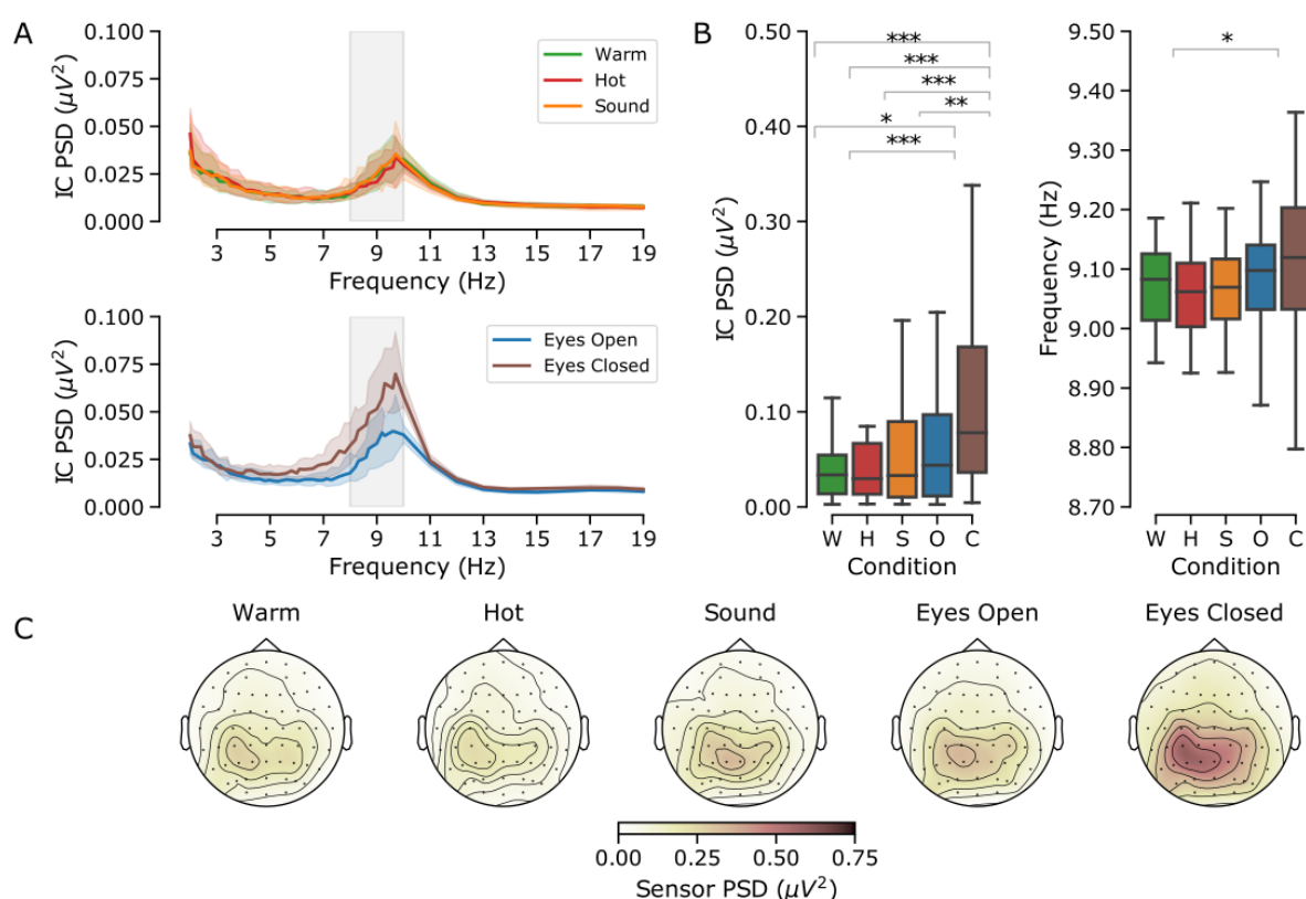
Figure 4. Slow alpha analysis (8-10 Hz). Panel A: grand-median (shaded area: 95% confidence interval) PSDs obtained following the IC alpha identification phase. Note how the alpha oscillations in the sensory stimulation conditions (upper graph) show lower magnitude and narrower frequency range than the baseline conditions (lower graph). Panel B: box-plots representing the median of individual average CoG power (left graph) and frequency (right graph) in all the five conditions (Warm, W, green; Hot, H, red; Sound, S, orange, Open eyes, O, blue, Closed eyes, C, brown). The boxes represent the inner quartiles while whiskers represent data within 1.5 times the inner quartile range. Data outside this range was not included in this figure. Asterisks represent statistical two-tailed significance (*** p < 0.001 , ** p < 0.01 , * p < 0.05 ). Note the expected progressive reduction of alpha magnitude from the baselines to the sensory stimulation conditions. Note also the reduction of frequency in the tonic hot condition compared with the eyes open baseline. Panel C: scalp topographies of mean power in the selected CoG frequency based only on the projection of the selected alpha ICs into sensors space.
