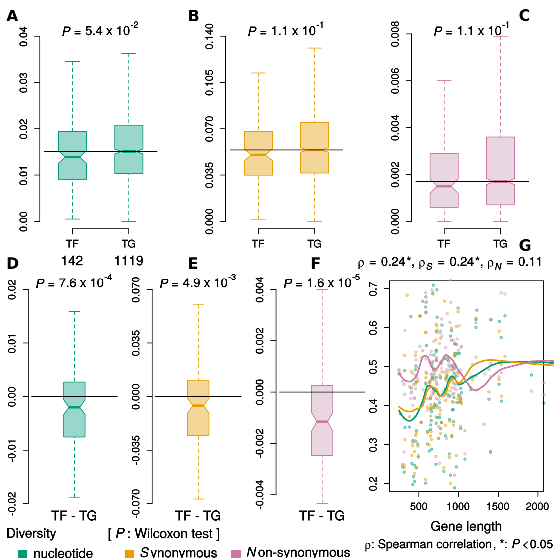
Fig. 1 Sequence diversity and gene length. A-C, Distributions of nucleotide, synonymous and non-synonymous diversity respectively, of TFs and TGs over 123 assembled genomes. D-F, Distributions of difference between the diversity of TFs and their own TGs for nucleotide, synonymous and non-synonymous diversity, respectively. Unpaired comparisons showed no significant difference but all paired comparisons did. G, Correlation between diversity difference (TF - TG) and TF's length. Nucleotide ( P = 0.0018 ) and Synonymous diversity ( P = 0.0023 ) were positively correlated with gene length, whereas Non-synonymous diversity was not ( P = 0.1016 ). Thick lines represent LOESS curves with a span of 0.5. Differences were Min-Max scaled for visualization. To improve resolution, outliers were excluded from box plots and y-axis for the scatter plot was restricted between 0.2 and 0.7 (which covers ~93 % of data points).
