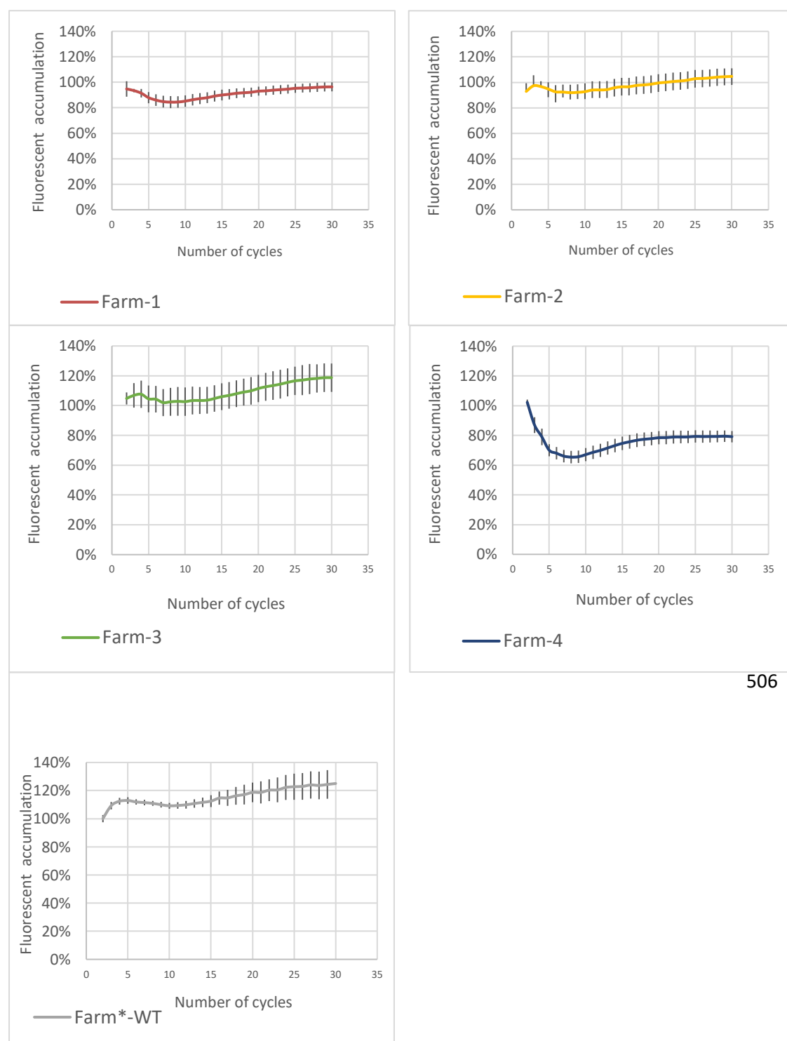
Figure 2. Envelope permeability of AmpC hyper-producing E. coli determined using fluorescent dye accumulation assays
