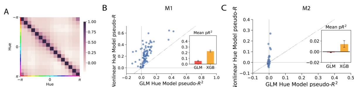
Figure S3. The response of V4 neurons to hue is nonlinear and contains interactions between bins of hues. A ) The correlation matrix of hues on the natural image dataset observed by M1. Since the off-diagonal terms are not zero, there are correlation between hues (especially of similar colors). These correlations could bias the tuning curve of a linear fit if nonlinear hue interactions exist in the neural response. As shown in (B) and in (C), these interactions do indeed exist. This can be seen by the fact that the nonlinear model (gradient boosted trees, XGB) predicts neural activity better than the generalized linear model (GLM) when both are fed the (saturation-weighted) histograms of hues present within the receptive field during each fixation.
