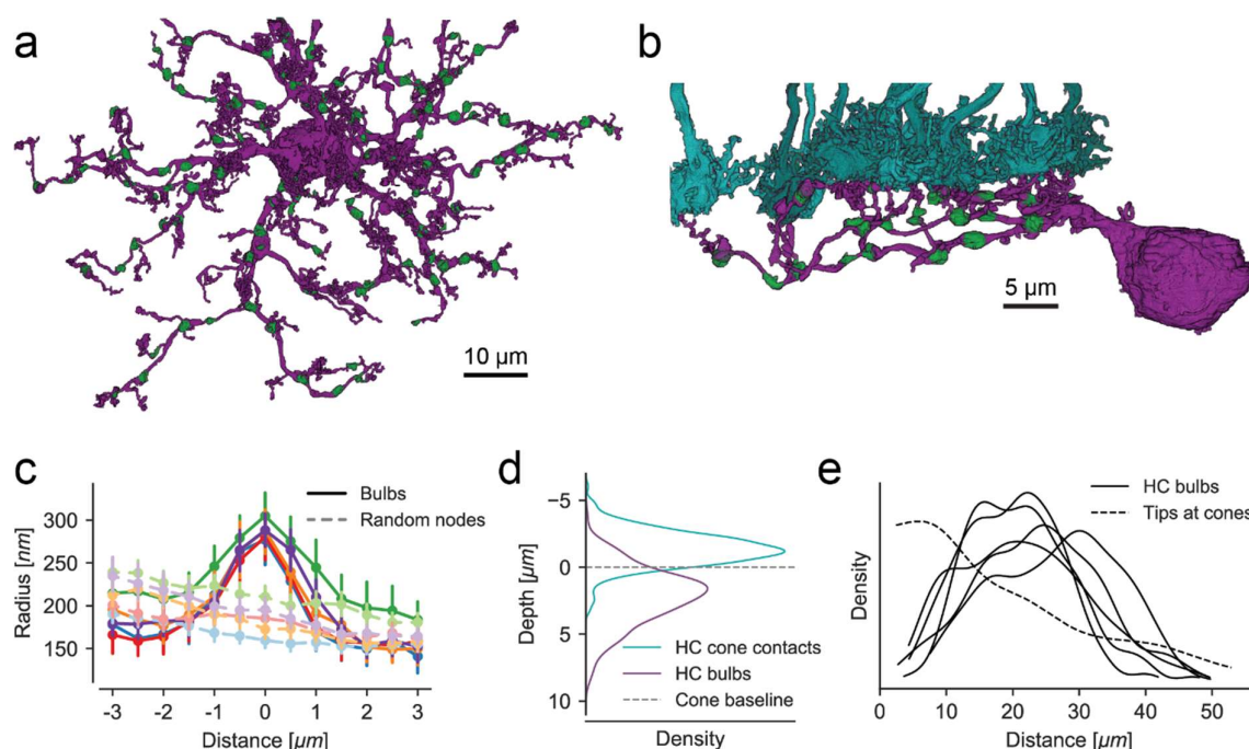
Figure 3. Identification of bulbs in horizontal cells. (a) Top view of a reconstructed HC with bulbs highlighted in green. (b) Side view of a branch from the same HC with bulbs (green) and cone axon terminals (cyan). (c) Dendritic radius profile at bulb locations (solid curves w/high saturation) compared to randomized points on the dendrites (dashed curves w/low saturation) with matching distribution of distances from soma and tips. (d) Depth of bulbs compared to HC-to-cone contacts. (e) Kernel density estimate of the distance distribution of bulbs relative to the soma for all five HCs. Dashed line: Model fit showing distribution of HC skeleton tips at cones from Fig. 2c.
