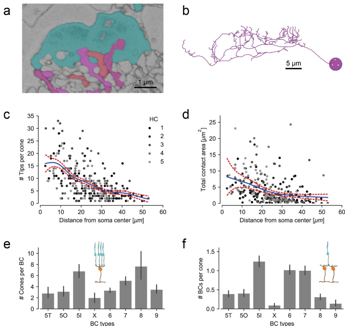
Figure 2. Horizontal cell-to-cone and HC-to-ON-CBC contacts (a) EM slice showing a cone axon terminal (cyan) with invaginating contacts from an ON-CBC (red) and a HC (magenta). (b) Vertical view of the skeleton model of the HC branch from Fig. 1e illustrating the increase of the number of dendritic tips towards the soma. (c) HC skeleton tips per contacted cone vs. distance from HC soma. Blue: Poisson GAM fit with 95%-confidence interval (red). (d) Contact area between HC and cone axon terminal volume reconstructions per cone vs. distance from HC soma. Blue: Gamma GAM fit with 95%-confidence interval (red). (e) Contacted cones per BC for all CBC types. (f) BCs contacted per cone for all CBC types. Number of ON-BCs contacting each cone per type. Both (e) and (f) redrawn using data from Behrens et al. 2016. Error bars show 95% CI.
