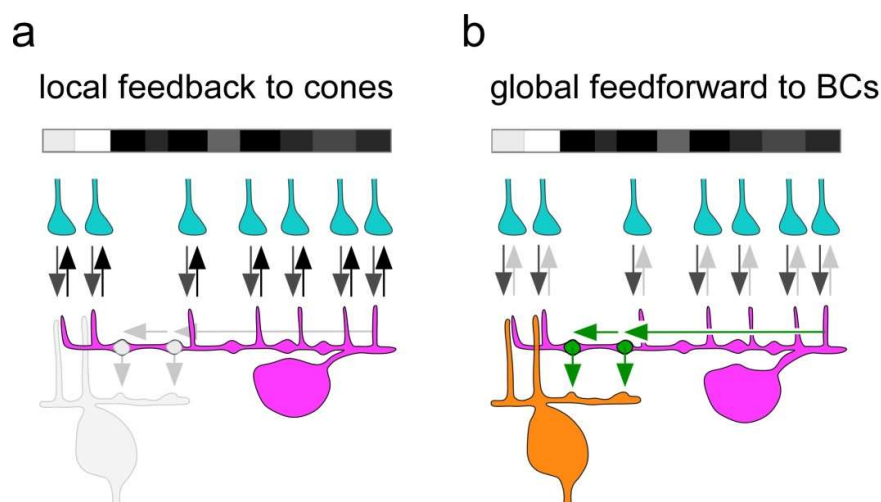
Figure 7. Synaptic circuitry of horizontal cells in the outer mouse retina. (a) Dendritic tips of a HC (magenta) receive cone input (grey arrows) and provide local and cone-specific feedback (black arrows) to cone axon terminals (cyan) in the presence of a spatially and temporally uncorrelated white noise stimulus (white/grey/black bar). (b) For the same uncorrelated stimulus, the cone input signals (grey arrows) are integrated to a global signal in the HC dendrite (green arrow) and forwarded by a BC-contacting bulb (green) to the BC (orange) forming the surround signal.
