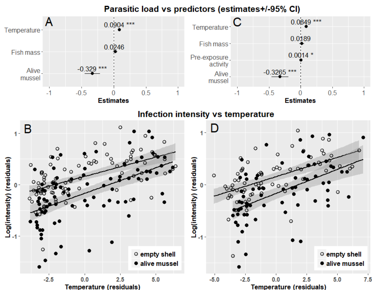
288 Fig. 1. Regression coefficients plots (A, C) and partial regression plots (B, D) showing the 289 influence of the temperature on the infection intensity in rainbow trout for the models fitted on the 290 full (A, B) and abridged dataset (C, D). In both cases, the presence of alive mussel in the container 291 caused a substantial decrease in the infection intensity in fish, while temperature increase led to 292 higher infection intensities. The regression lines for containers with alive mussels and control 293 containers are almost parallel, confirming the lack of interaction between the temperature and 294 presence of alive mussel in the environment. Fish, which were more active prior to the exposure, 295 were more infected compared with less active fish (A, C) (about 15% increase in the infection 296 intensity per 100 additional lines crossed by fish in five min).
