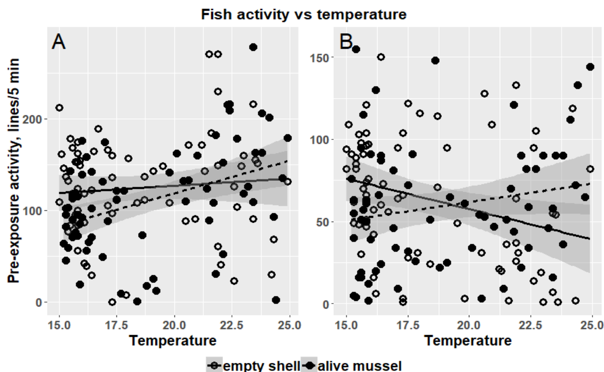
Fig. 3. Rainbow trout pre-exposure (A) and post-exposure (B) activity depending on temperature. (A) Before the exposure to parasites, fish activity increased with temperature both in the presence of the alive mussel and in the control (empty mussel shell) (Estimate±SE = 4.27±1.47 for the similar slopes model). Though the slopes of regression lines for both groups did not differ significantly ( p = 0.06 ), the line for fish in the presence of alive mussels was steeper (dashed line). (B) After exposure, the slopes of regression lines became significantly different. In the presence of alive mussels, fish still increased their activity with increasing temperature, while in the control, fish decreased their activity with temperature. Temperature influenced the degree of activity change after the exposure to cercariae, i.e. pre-exposure activity minus post-exposure activity (Estimate±SE = 4.95±1.67, t = 2.97 , p = 0.004 , Fig. 4), while the addition of treatment (alive mussel/empty shell) and the interaction in the model did not increase additional amount of variance (Fig. 4). Fish changed their activity more under high temperatures compared with low temperatures.
