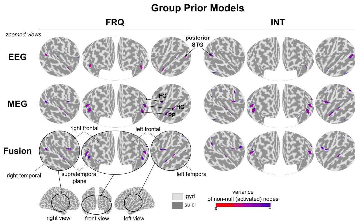
Figure 5. Comparison of group prior models obtained for EEG, MEG and fusion (in separate rows), with the frequency (left panel) and intensity (right panel) deviances. For each modality and each condition, three zoomed views (with relation to the global view indicated at the bottom left) indicate the result of MSP inversion performed at the group level (first step of group-level inference), hence reflecting the source distribution common to the group.
