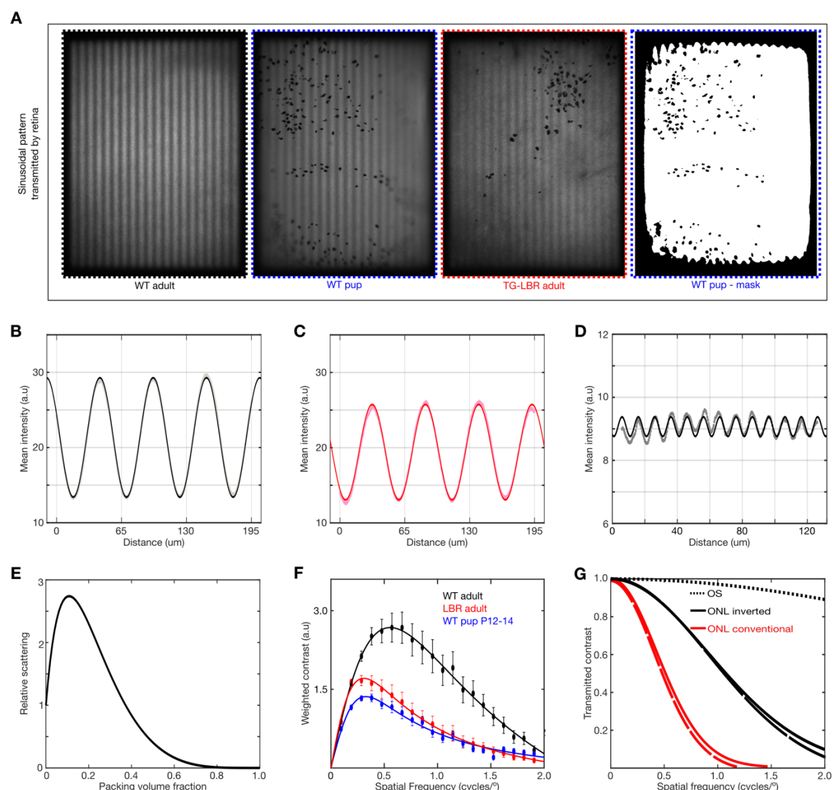
Fig. S6. Modulation Transfer Function and its relation to light scattering and visual perception.
