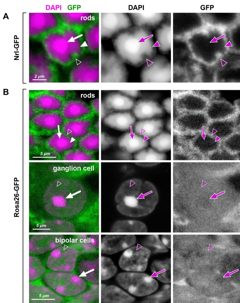
Fig. S3. Heterochromatin in rod nuclei exhibits unusual dense packing.
