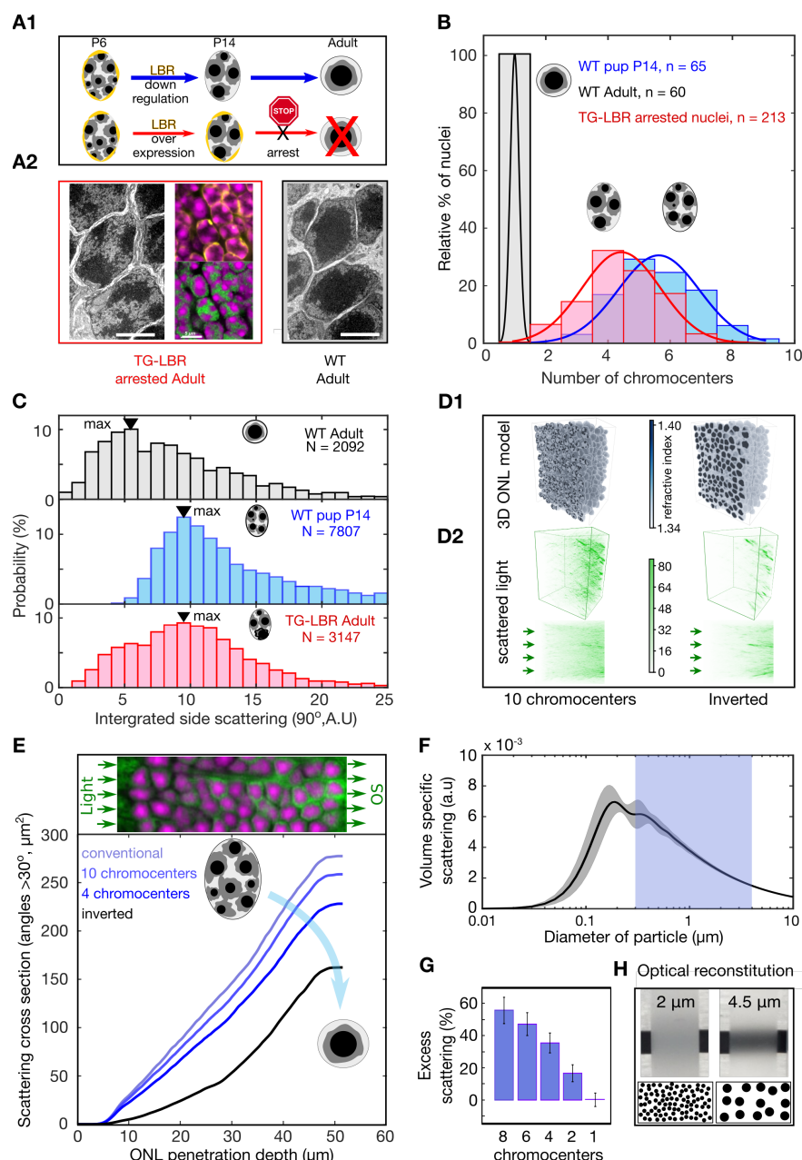
Fig. 2 Developmental arrest of chromocenter fusion increases light scattering from rod nuclei in measurements and tissue simulations. (A1) Schematic of the normal rod nuclear WT development and inversion arrested nuclei by LBR overexpression. (A2) EM images illustrating different electron densities in the euchromatic and heterochromatic phase underlying their refractive index (RI) differences (scalebar 5μm). (mid-top) Immunostaining of overexpressed of LBR tethers (yellow), and high-density heterochromatin (DAPI, magenta). (mid- bottom) Heterochromatic chromocenters (DAPI, magenta) and euchromatin (H4K5ac, green) (B) Chromocenter number distribution in LBR overexpressing rod nuclei is drastically different from WT mice, and similar to a developing WT pup (P14). (C) Side scattering assessed by FACS for TG-LBR retina nuclei is higher than that of WT nuclei and comparable to that of a WT P14 nuclei with similar chromocenter numbers. Note the shift of peak value upon LBR overexpression. (D1) 3d RI distribution mapped onto anatomically faithful volumetric ONL images. WT inverted architecture (right, top) and early developmental state (left) (simulation). (D2) (top) Differential simulations of light propagation in the ONL, using same positions and shapes of about 1750 nuclei, but varying chromatin distributions. (bottom) Maximum projection illustrating greater proportions of scattered light (angles >30deg) in the ONL with multiple chromo-centered nuclei. (E) Quantitative analysis of this data. (F) Angle weighted volume specific scattering strength for nuclei models evaluated by Mie scattering theory. (G) Excess scattering occurring in multi-chromocenter nuclei models. (H) Chromocenters scattering reconstituted in an emulsion of silica spheres in glycerol-water mixture. Pictograms reflect accurate number ratio of spheres.
