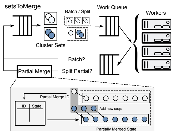
Figure 5. High-level architecture of Dist-CM.
