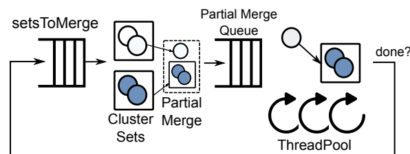
Figure 4. High-level architecture of Shared-CM.
