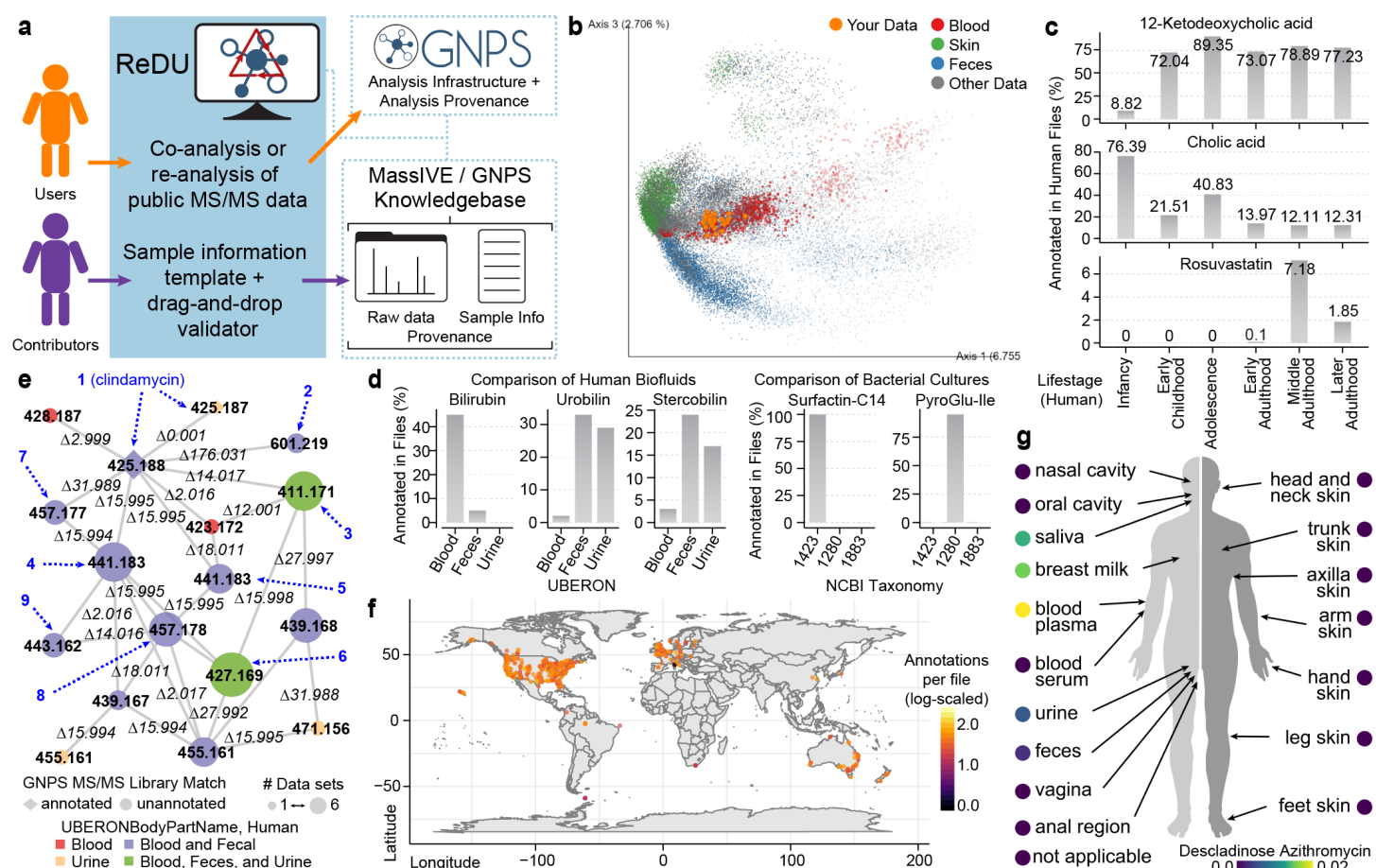
Fig 1. ReDU workflow and illustrative applications. (a) The ReDU framework. (b) Users can co-analyze their data via projection onto public data visualized using EMPor 11 . PCA was performed on GNPS annotations (level 2/3). 7 Human blood plasma samples (orange) from rheumatoid arthritis patients. Sample points size and color were set using UBERON ontology and opacity was set using NCBI taxonomy filtering (your data, 1.0; 9606|Homo sapiens, 0.7; and all other data, 0.25). (c) Metadata filters were used to select human fecal samples (NCBI taxonomy, 9606|Homo sapiens; UBERON, feces) and launch sample information enrichment. Chemical explorer
