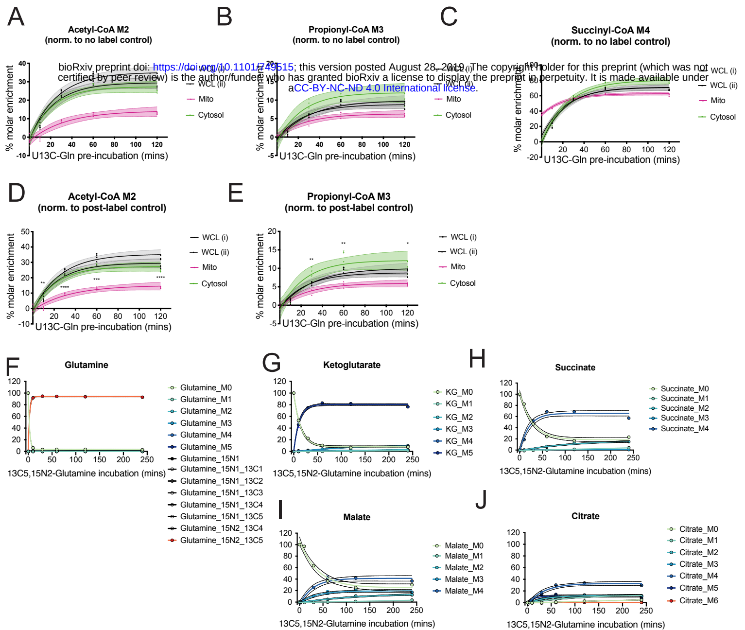
Supplemental Figure 4: Kinetics of glutamine metabolism in the mitochondria are transformed by post-label correction HepG2 cells were pre-labeled over a time-course with 2 mM ^{15}\text{N}_2^{13}\text{C}_5 -glutamine. Absolute isotopologue enrichment of mito/cyto fractionation post-labeled data when normalized to no label control for acetyl-CoA M2 ( A ), propionyl-CoA M3 ( B ) and succinyl-CoA M4 ( C ). Acetyl-CoA M2 ( D ) and propionyl-CoA M3 ( E ) post-labeled data when corrected by normalization to post-labeled control. F-J Isotopologue analysis of tricarboxylic acid (TCA) cycle intermediates after direct extraction from whole cells. Data from representative experiments is shown. Shading indicates 95% confidence bands and symbols represent individual replicate values (n=3). For comparison between two groups, datasets were analyzed by student's t-test with statistical significance defined as p < 0.05 (*), p < 0.01 (**), p < 0.001 (***), p < 0.0001 (****).
