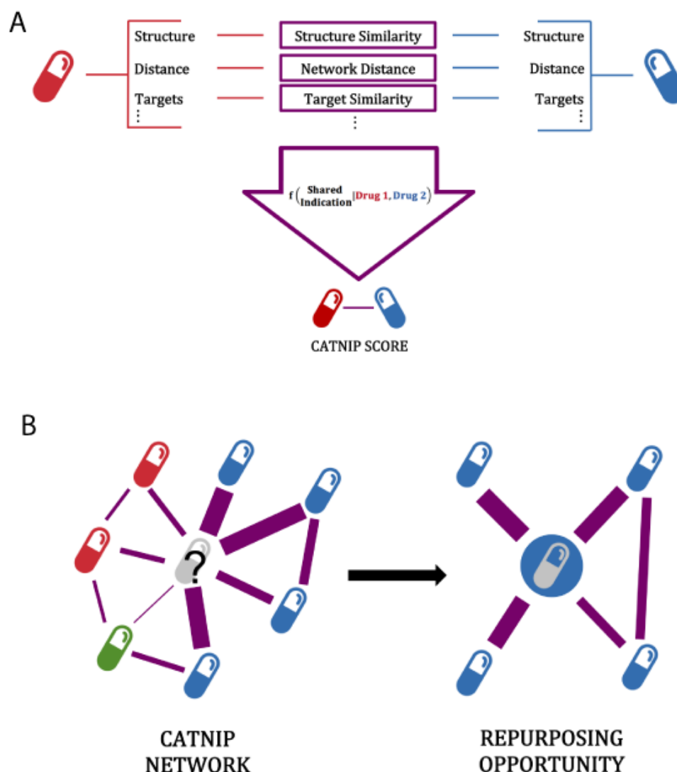
Figure 1: Schematic of CATNIP repurposing approach. A) The use of drug similarity properties to predict if two drugs will share an indication using a gradient boosting model, the model is referred to as CATNIP. B) Schematic showing the use of CATNIP output scores to create a network, with the scores used as edge weights. The colors of each drug represent the known disease and this demonstrates how one could identify novel indications for drugs through the network.
