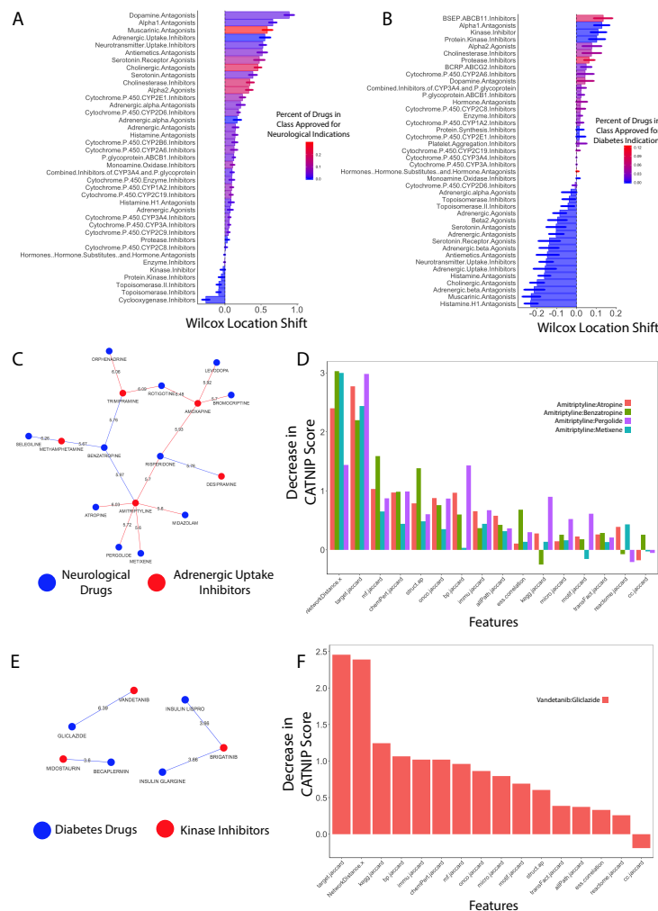
Figure 3: CATNIP identifies drug class repurposing opportunities. The location shift, calculated using Wilcoxon-Mann-Whitney for all CATNIP scores of drug class-disease drug pairs vs drug class-non-disease drug pairs for A) “neurological diseases” and B) “diabetes”. Drug classes are colored based on the percent of drugs within the class that are approved for treatment of the specific disease and only significant associations are shown (FDR < 0.1). C) The network of neurological drugs and adrenergic uptake inhibitors drug pairs with the highest CATNIP scores. D) The decrease in the CATNIP score when removing each feature for amitriptyline and select Parkinson’s Disease drugs. E) The network of anti-diabetes and kinase inhibitor drug pairs with the highest CATNIP scores. F) The decrease in the CATNIP score when removing each feature for the drug pair vandetanib and gliclazide.
