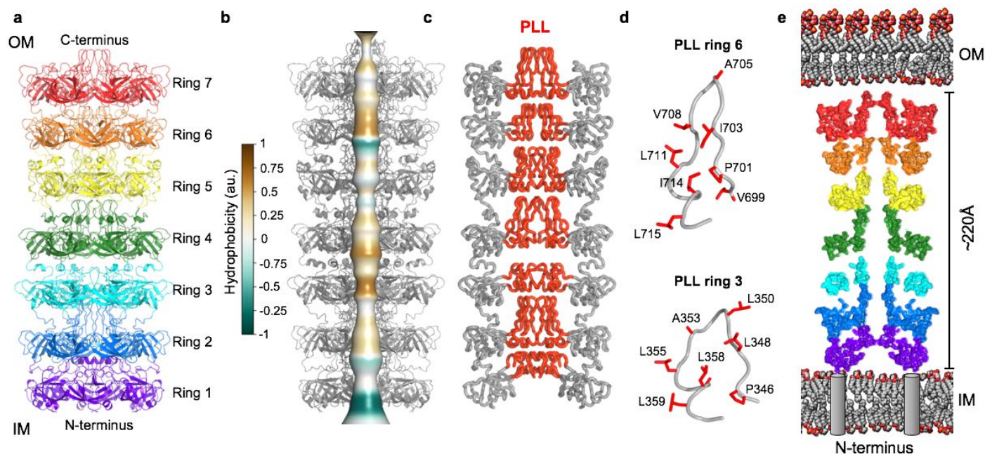
Figure 2. LetB hexamers form a tunnel. a. Cartoon representation of a LetB hexamer showing 7 stacked rings, each formed from the association of 6 identical MCE domains. b. Composite model of LetB in the open state (further described in Fig. 4 and associated text), showing tunnel running through the protein assembly. Tunnel is depicted as smooth surface coloured by the hydrophobicity of pore-facing residues, calculated using CHAP 54 . c. Ribbon representation of LetB. Pore-lining loops (PLLs; red) from each MCE domain form the central tunnel. d. Representative PLLs (PLL3 and PLL6) with pore facing residues shown as red sticks. Most pore-facing residues are hydrophobic. e. Cross-section of the LetB tunnel oriented in the context of the IM and OM, with the N-terminus anchoring the complex in the IM and the C-terminus towards the OM. Grey cylinders represent transmembrane helices (TM, not present in the structure) at their expected positions. The width depicted between the IM and OM is within a range of 210–240 Å, based on previously measured periplasmic widths, 210 Å 22 and 230 Å 21 , and deduced from the periplasmic spanning region of AcrAB-TolC, 240 Å 59 .
