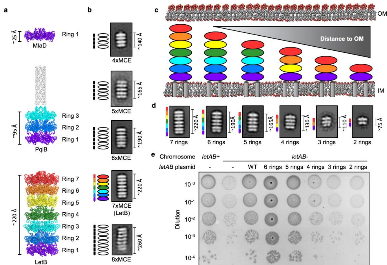
Figure 3. MCE domains are modular building blocks that determine the length of MCE protein assemblies. a , Cartoon representations of E. coli MCE proteins MlaD (PDB ID: 5UW2), PqiB (PDB ID: 5UVN) and LetB, which contain one, three and seven MCE domains, respectively, and form architectures with the corresponding number of rings. b , Negative stain EM 2D class averages of naturally occurring proteins encoding four, five, six, seven (LetB), and eight MCE domains (Extended Data Fig. 6). Schematics to the left of 2D class averages indicate number of MCE domains present in the gene (rectangles) and expected number of rings based on modularity of MCE domains (ovals). c , Truncated constructs designed to modulate number of LetB rings and their expected length in the context of the periplasm. As number of LetB domains is reduced, distance to OM is predicted to increase. Colour coding is the same as in a ; see Methods for rationale of construct design. d , Negative stain EM 2D class averages of LetB truncation mutants depicted in c , but with the TM helix deleted for each mutant. Domain organisation of the gene is shown to the left of the 2D class average. The 7 ring 2D class average is the same as the 7xMCE class in (b) . e , Cellular assay for the function of LetB truncation mutants depicted in c . 10-fold serial dilutions of the indicated cultures spotted on plates containing LSB and incubated overnight. The letAB double mutant grows poorly in the presence of LSB, but can be rescued by the expression of letAB constructs containing letB encoding five, six, or seven (WT) MCE rings. Expression of constructs with letB containing two, three, or four rings fail to rescue.
