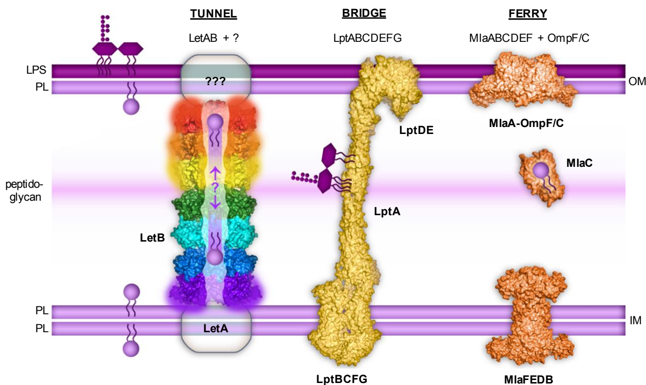
Figure 6. Model for LetB function in lipid transport. LetB forms a tunnel capable of spanning the periplasm, potentially interacting with LetA in the IM and unknown partners in the OM. Rings 1, 5, 6 and 7 are dynamic and adopt open and closed states (indicated by blurring). Lipids are transported through the tunnel, though the direction of transport remains unknown. Two other lipid transport systems in E. coli are depicted: 1) The LPS transport system, which is composed of Lpt proteins (PDB IDs: 5iv9, 2r1a and 6mit), forms a bridge between the two membranes along which LPS is transported; and 2) The Mla system, another MCE-protein family member (PDB IDs: 5nup, 5uwa and EMD 8610), which is composed of IM and OM complexes, and a soluble protein, MlaC, which “ferries” lipids across the hydrophilic periplasm. These three systems employ fundamentally different mechanisms for lipid transport, analogous to tunnels, bridges, and ferries.
