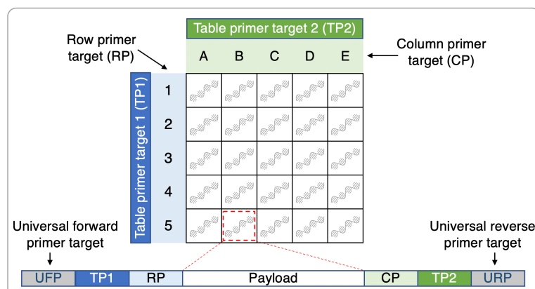
Figure 3. Multidimensional data organization and design of data-encoding strands in design B.
