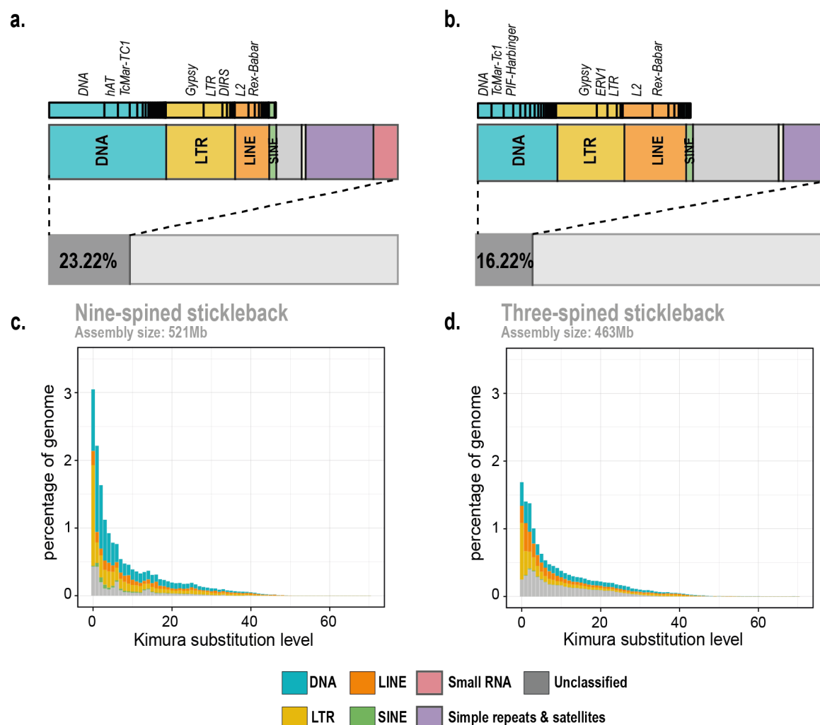
Fig. 2: Transposable elements in stickleback genomes. a and b represent the fraction of the assembly comprising of repetitive elements in nine- and three-spined stickleback (Glazer et al. 2015) assemblies, respectively. Repeat landscapes representing the divergence of the repeat sequences to the consensus are represented for nine- and three-spined stickleback genomes in c and d respectively.
