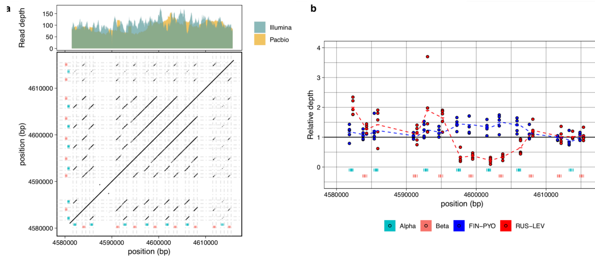
Fig. 6: Analysis of hemoglobin MN cluster. a. Dotplot (bottom) representing self-alignment of the MN cluster region of the hemoglobin in nine-spined stickleback. Top: Mapped read depth across the MN cluster of hemoglobin in nine-spined stickleback. b. Relative read depth for five individuals each from nine-spined stickleback populations FIN-PYO (Pyöreälampi pond, Finland) and RUS-LEV (Levin Navolok Bay, Russia). The dashed lines connect the means of the read depth for each of the hemoglobin genes.
