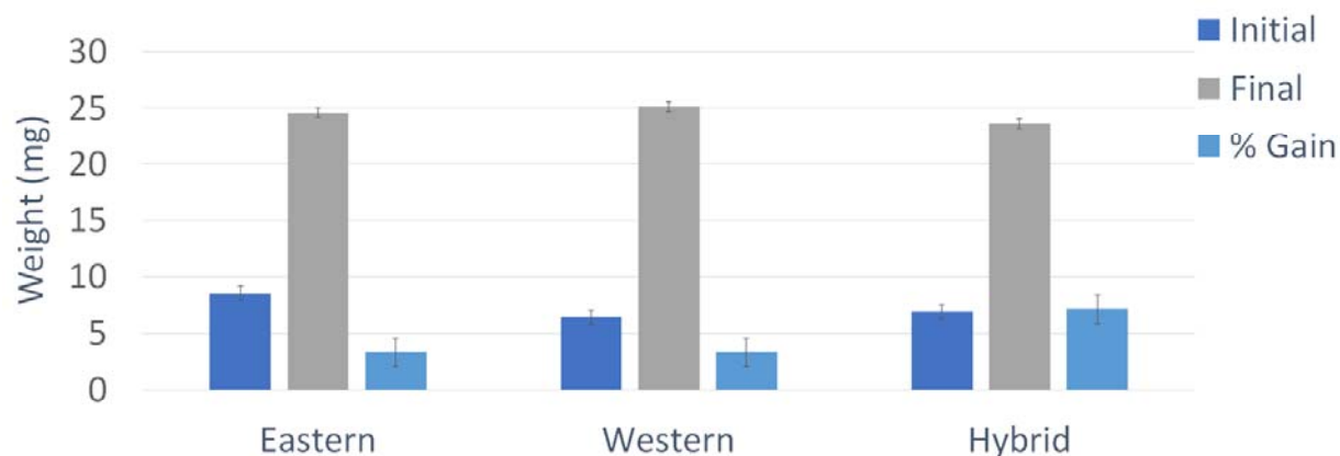
Fig. 1 Weight in mg (initial, final), and percentage weight gain from aphid utilization in Eastern, Western, and Hybrid populations of Hippodamia convergens when an individual larva was placed per plant, across eight replicate treatments.
