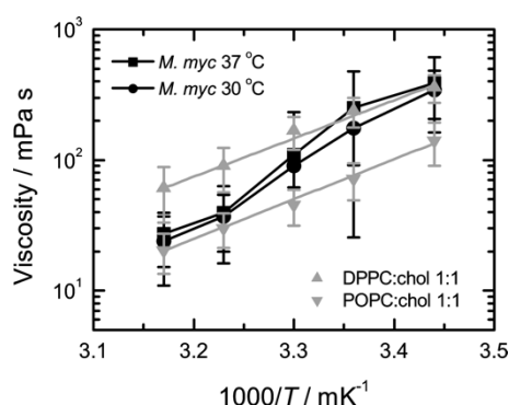
Figure 7. Influence of temperature on viscosity of native lipid membranes from M. mycoides grown at 30 and 37 °C (n=5). For comparison, viscosities (symbols) of Ld (POPC/cholesterol 1:1) and Lo (DPPC/cholesterol 1:1) membranes are plotted with corresponding fit of the Arrhenius law (lines).
