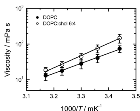
Figure 4. Viscosity of lipid membrane composed of DOPC and DOPC/cholesterol 6:4 (mol:mol). Viscosity data are shown with a fit using the Arrhenius law (line). The activation energies were 54 \pm 9 and 63 \pm 8 kJ/mol for pure and cholesterol doped DOPC membrane, respectively.
