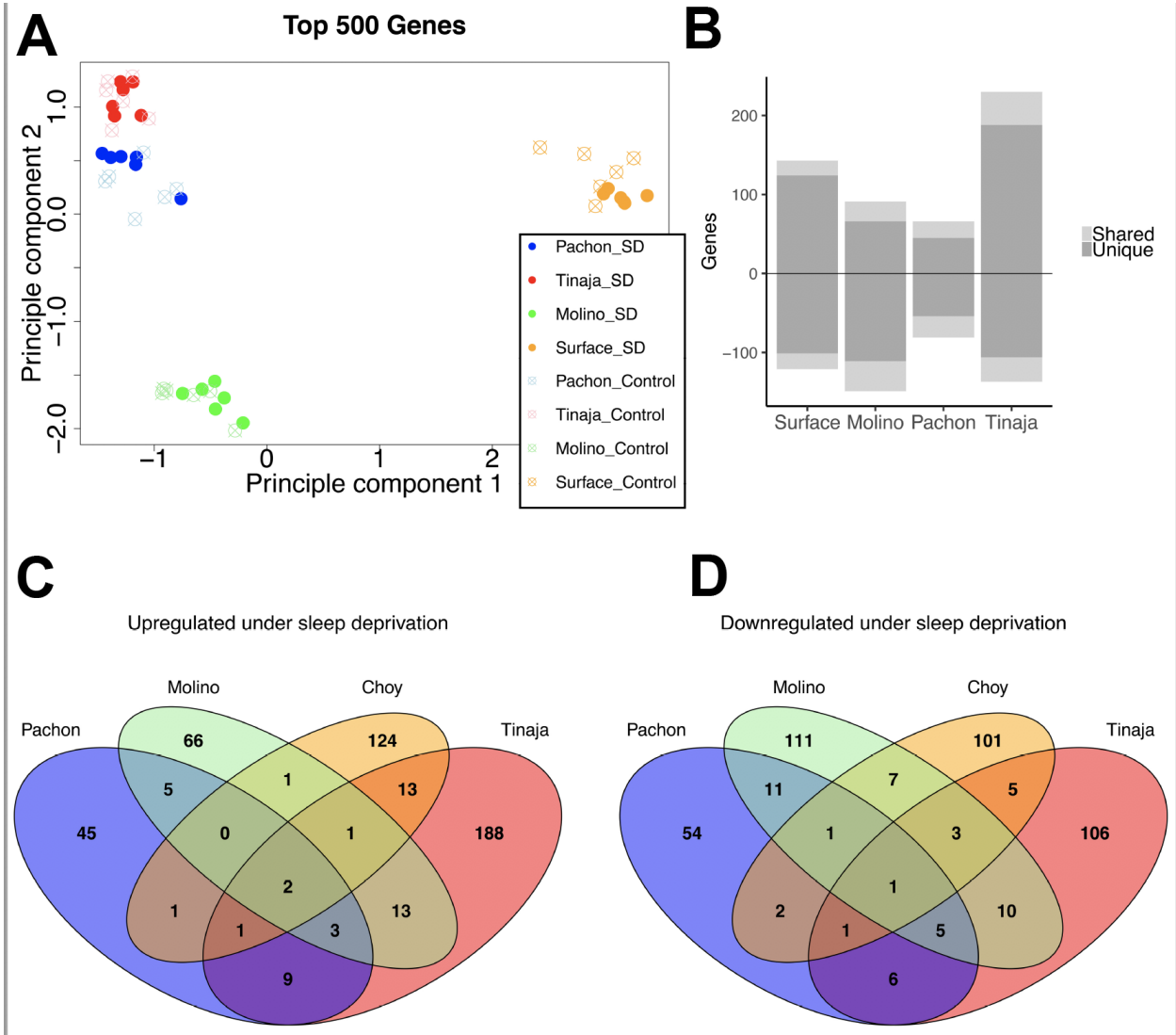
Figure 3. A) MDS plot of 500 Top genes between control and sleep deprivation treatments the four populations normalized for library size. PC1 clearly demarcates population of origin. B) Number of genes differentially expressed between control and sleep deprived treatments. Above zero is upregulated in sleep deprived samples and below zero is downregulated in sleep deprived samples. Light grey = shared with at least one other population, Dark grey = not shared among other populations. Overall few genes are differentially expressed in response to sleep deprivation and differentially expressed genes are not shared among populations. C) Venn-diagram of overlap in differentially upregulated genes in the sleep deprivation treatment between all four populations. D) Venn-diagram of overlap in differentially downregulated genes in the sleep deprivation treatment across all four populations.
