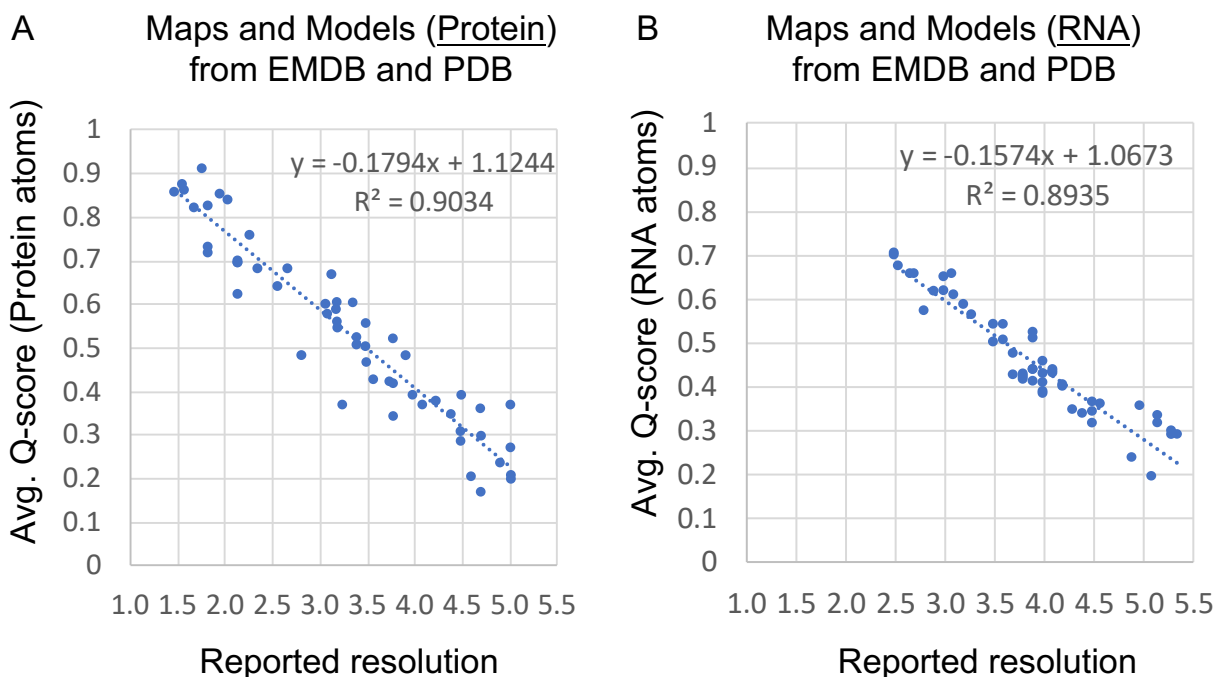
Figure 5. Model Q-scores compared to reported resolution for maps and models obtained from EMDB. (A) Average Q-scores for atoms in proteins. (B) Average Q-scores for atoms in RNA.
