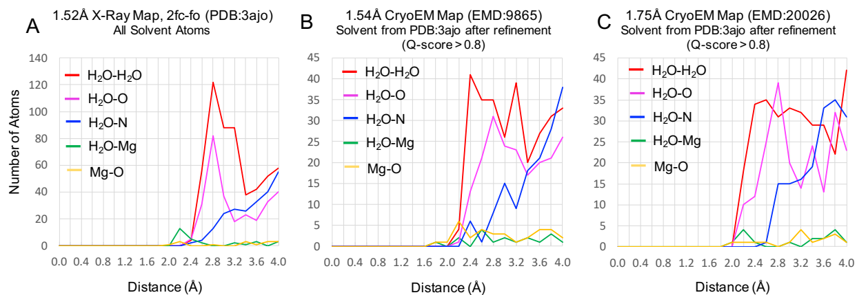
Figure 8. Radial plots of distances from solvent atoms to other types of atoms. Oxygen atoms in water are labeled \text{H}_2\text{O} , whereas oxygen/nitrogen atoms in protein are labeled O/N respectively.
