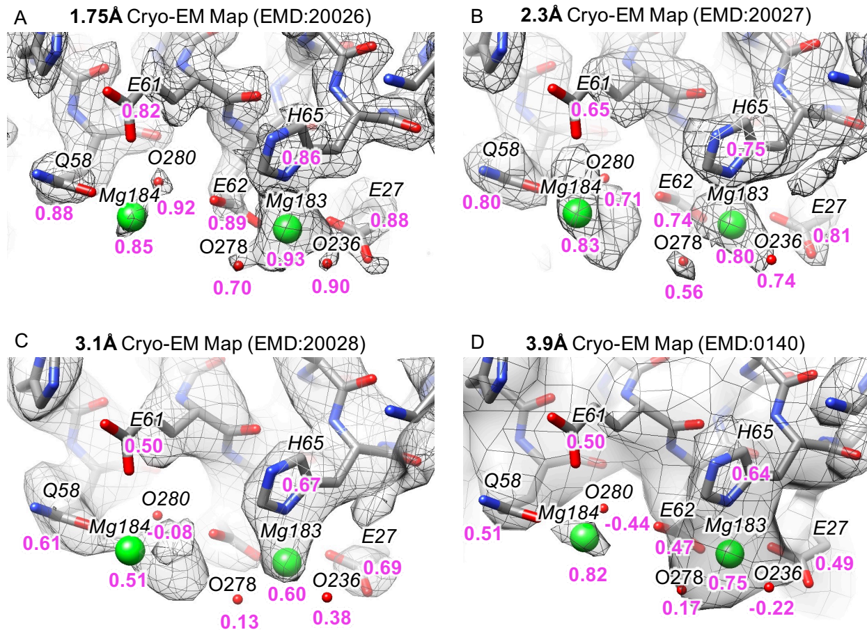
Figure 9. Solvent atoms from X-ray model (PDB:3ajo) in cryoEM maps at resolutions of 1.75Å to 3.9Å. Q-scores are shown in purple below each atom. Nearby residues with Q-scores are also labeled (Q58, E61, E62, H65, E27).
