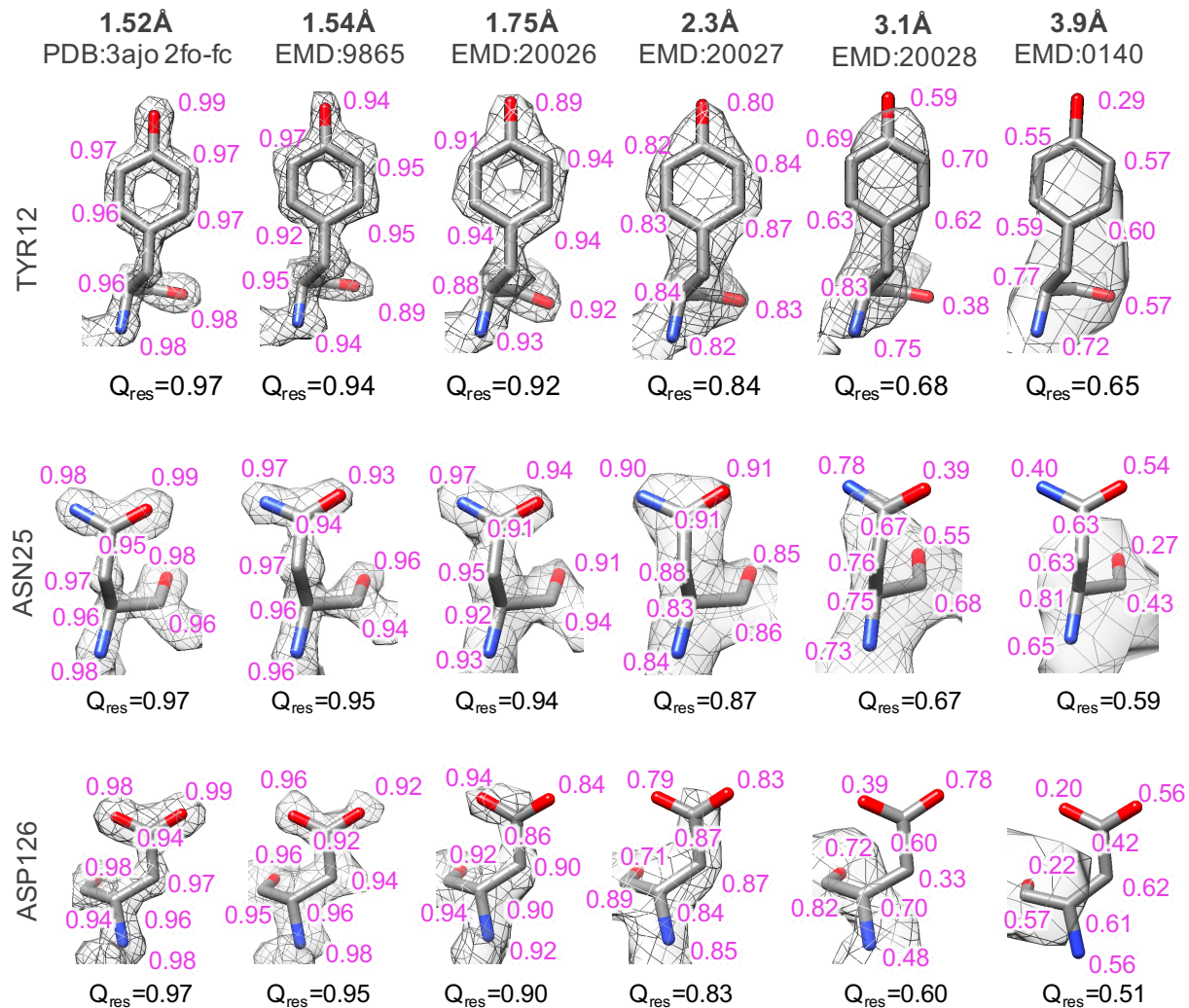
Figure 3. Atom Q-scores for three types of residues, taken from Apoferritin maps at various resolutions. Atom Q-scores are shown in purple close to each atom.
