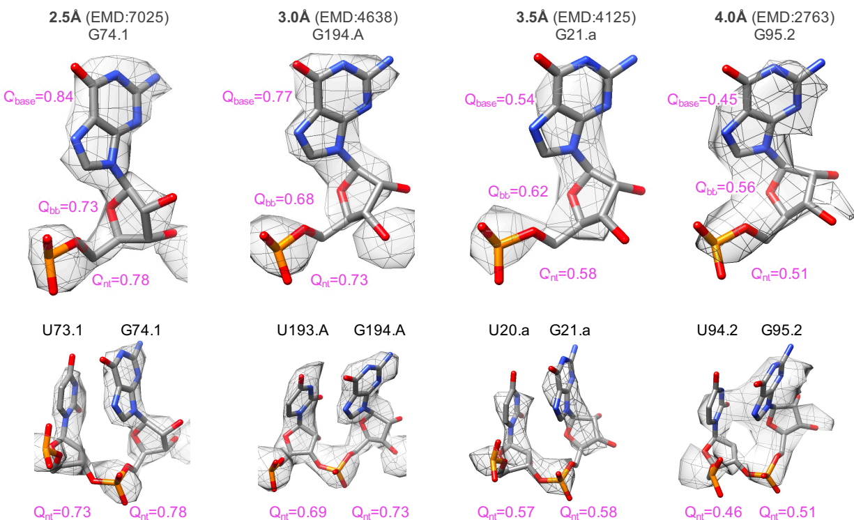
Figure 4. Q-scores averaged over entire nucleotides ( Q_{nt} ) in RNA maps and models from the EMDB at four different resolutions. Q-scores are also averaged for the base ( Q_{base} ) and phosphate-sugar backbone ( Q_{bb} ) groups in the nucleotides shown on the top row.
