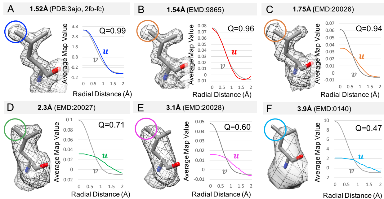
Figure 2. Calculation of Q-scores for an atom in 6 maps at different resolutions, including an X-ray map. The atom is CD2 from Leu 26 in PDB:3ajo. The atomic profile in each map is marked with the letter u , while the reference Gaussian is marked with v .
