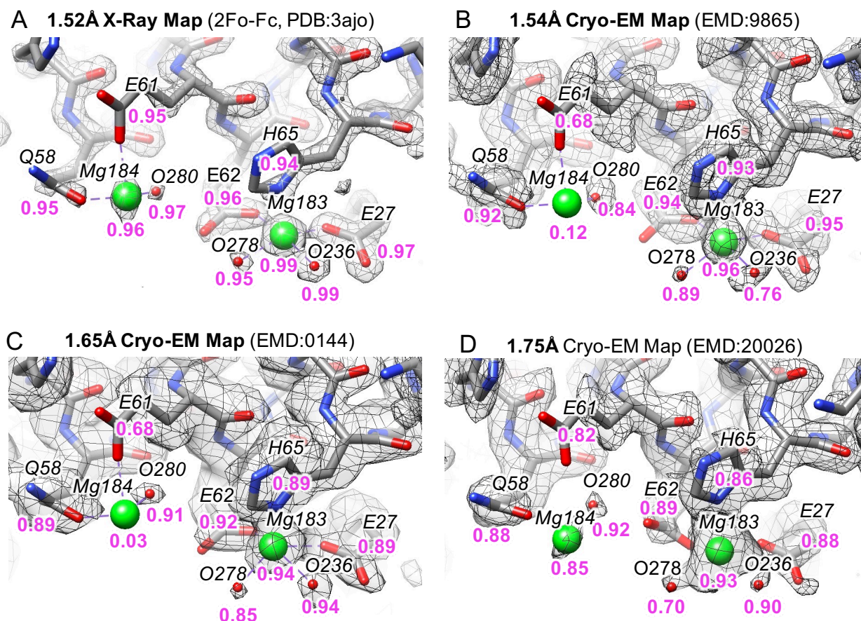
Figure 6. A close up in Apoferritin models showing solvent atoms (Mg and O from water), along with calculated Q-scores in purple under each atom and nearby residue. The model comes from the X-ray map (PDB:3ajo) shown in A. It was further refined into each of the three cryoEM maps, B-D.
