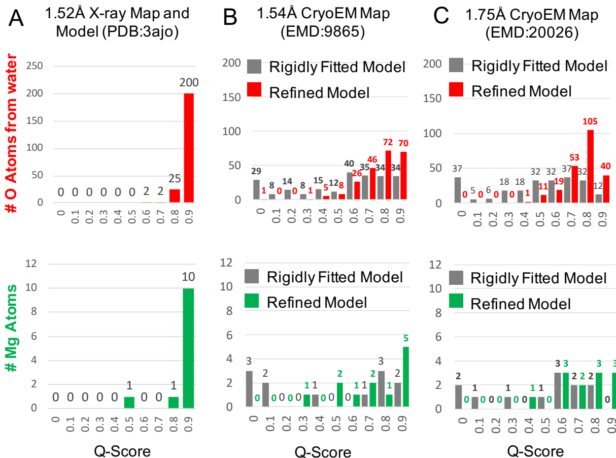
Figure 7. Distribution of Q-scores for solvent atoms (water and Mg) in X-ray map (PDB:3ajo), and in two cryoEM maps before and after refinement.
