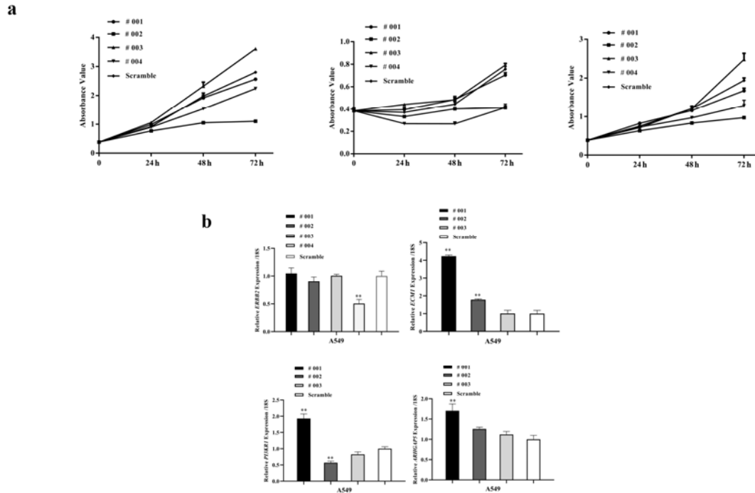
Figure 4 The effects of #001–#004 miRNA expression cassettes on cell proliferation and the target genes. (a) The effects of #001–#004 miRNA expression cassettes on cell proliferation, as related to the state of p53 activation, with the addition of doxorubicin and nutlin3. (b) Target gene ( ErbB2 , ECM1 , PI3KR1 , and ARHGAP5 ) expression, as reported by previous studies, was regulated by miR-125a-5p, miR-486-3p, and miR-486-5p, respectively, in stable A549 cell lines, which expressed the #001–#004 miRNA expression cassettes. The cell line that stably expressed the scramble sequences were used as negative controls. * P < 0.05 and ** P < 0.01 (Student's t -test). The data are from three independent experiments (mean \pm SEM).
