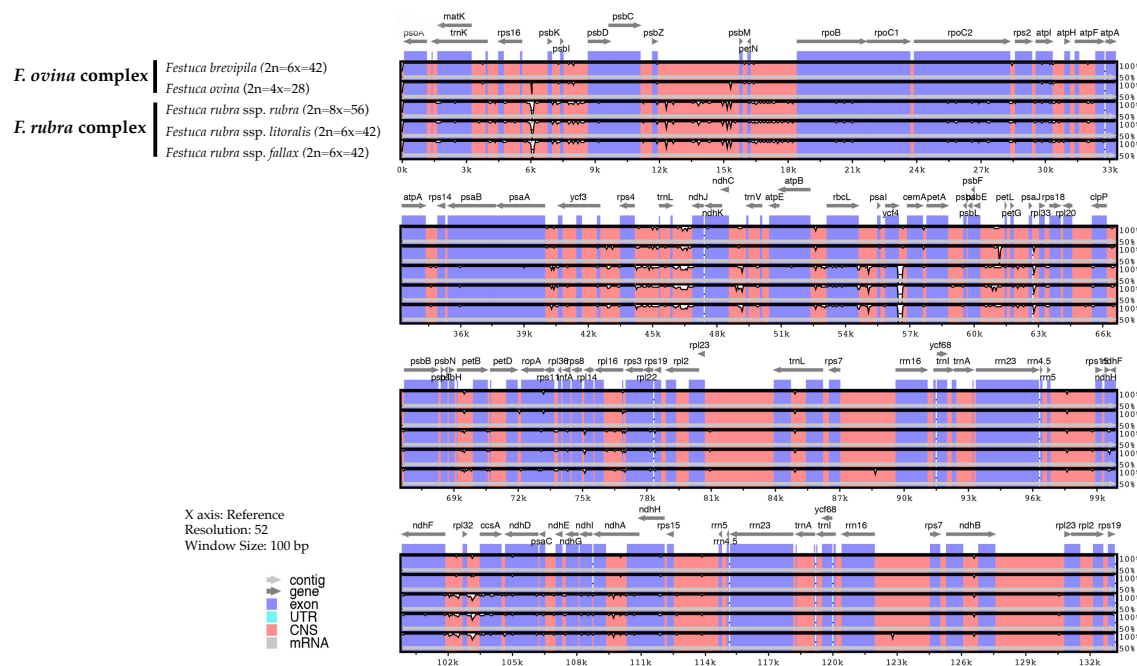
Figure 4. Sequence identity plot of fine fescues chloroplast genome sequences with F. ovina (2x) as the reference using mVISTA. A cut-off of 70% identity was used for the plots, and the percent of identity varies from 50% to 100% as noted on the y-axis. Most of the sequence variations between fine fescues were in intergenic regions. Taxa in the F. ovina complex, F. brevipila and F. ovina showed high sequence similarity. Similarly, subspecies within F. rubra complex also showed high sequence similarity.
