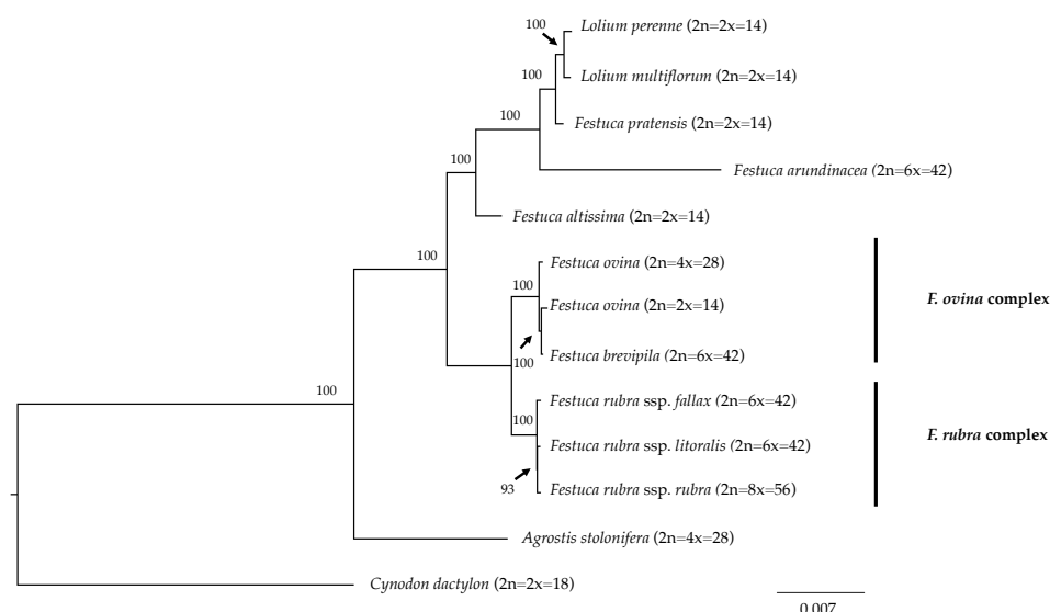
Figure 8. Maximum likelihood (ML) phylogram of the Festuca - Lolium complex with 1,000 bootstrap replicates. Fine fescues were grouped into previous named complexes ( F. ovina and F. rubra ), sister to broad leaved fescues in the Festuca - Lolium complex.
