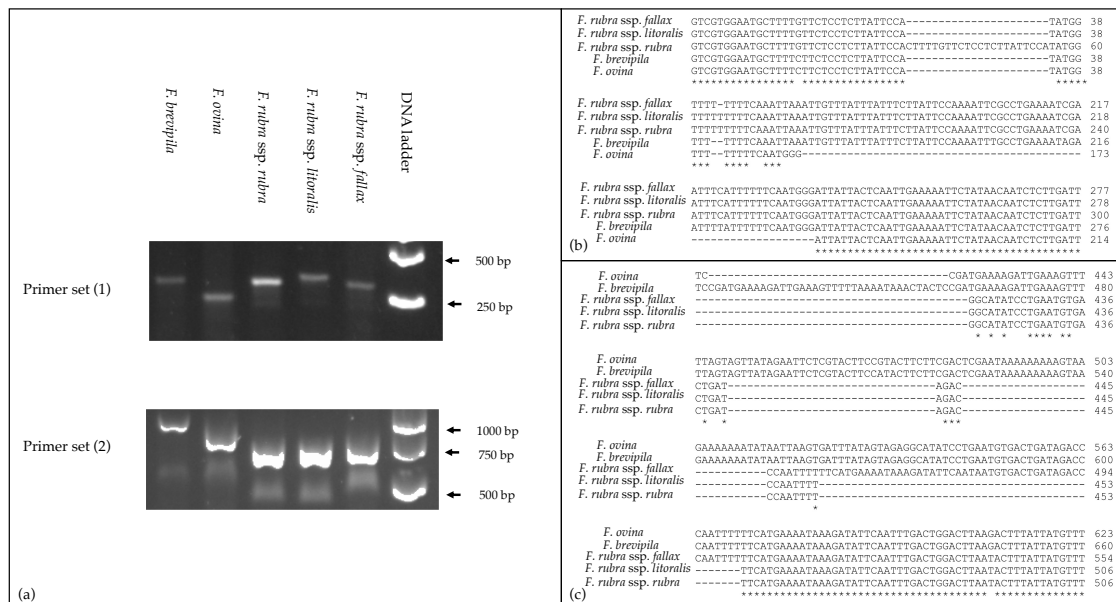
Figure S2. Examples of PCR validation of predicted repeat regions based on fine fescue chloroplast genomes. PCR primers were developed using Primer3 module(Untergasser, Cutcutache et al. 2012). Primers used for the PCR assays (1) Forward primer 5'-GTCGTGGAATGCTTTTGTCTC-3'; Reverse primer 5'-AGTGGATTTCATCAGATGATACA-3'; (2) Forward primer 5'-TTCCTCTTTTCATTGCAAAGTGGT AT-3'; Reverse primer 5'-TACTCGGAGGTTTCAATCCTTCC-3'. PCR products were examined on 1% agarose gel and gel images showed fragment size separation between different taxa(a). Figure (b) and (c) showed partial sequence alignment of regions amplified by primer sets (1 and 2).
