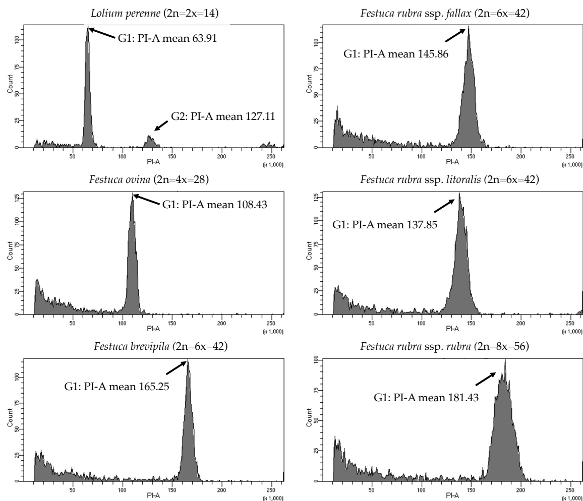
Figure 1. Flow cytometry results for the five fine fescue taxa. Lolium perenne ( 2n=2x=14 ) was used as the reference. Flow cytometry was able to separate F. rubra ssp. rubra from the other two subspecies
