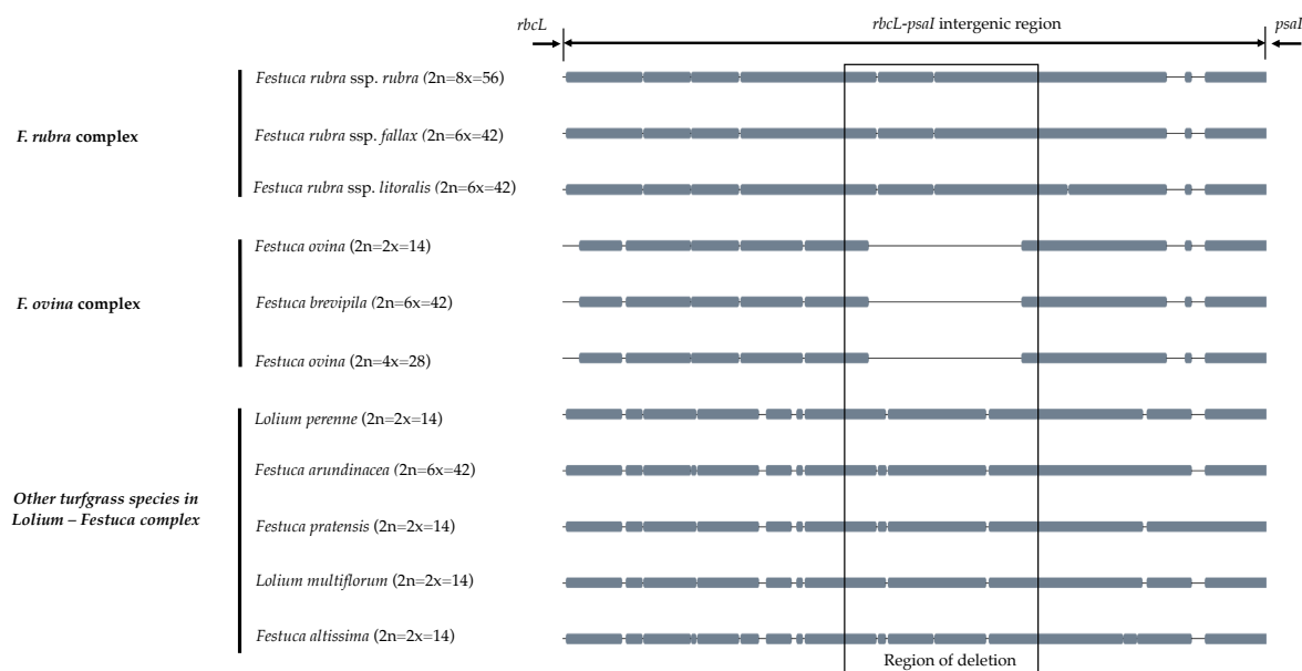
Figure 7. The alignment of rbcL-psaI intergenic sequence shows that the pseudogene accD is missing in both F. ovina (2x, 4x) and F. brevipila but present in the F. rubra complex and other species examined in this study. Species were ordered by complexes.
