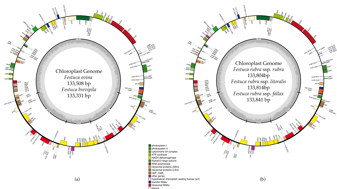
Figure 2. Whole chloroplast genome structure of F. ovina complex (a) and F. rubra complex (b). Genes inside the circle are transcribed clockwise, genes outside are transcribed counter-clockwise. Genes belong to different functional groups are color coded. GC content is represented by the dark gray inner circle, the light gray corresponded to the AT content. IRA(B), inverted repeat A(B); LSC, large single copy region; SSC, small single copy region.
